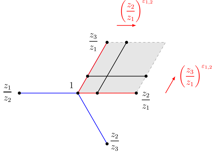
FIGURE 1. \mathcal{N}((1 - z_3/z_1)(z_2/z_1)^{\varepsilon_{1,2}}) , \mathcal{N}((1 - h z_2/z_1)(z_3/z_1)^{\varepsilon_{1,2}}) are contained in \mathcal{N}((1 - z_2/z_1)(1 - z_3/z_1)) .
