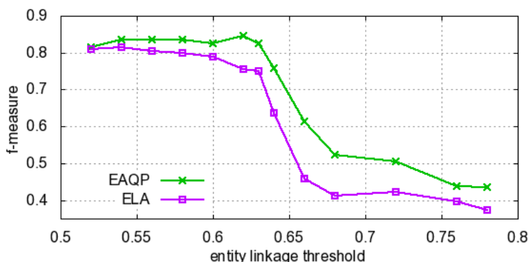
Figure 4.2: F-measure for EAQP and ELA.
