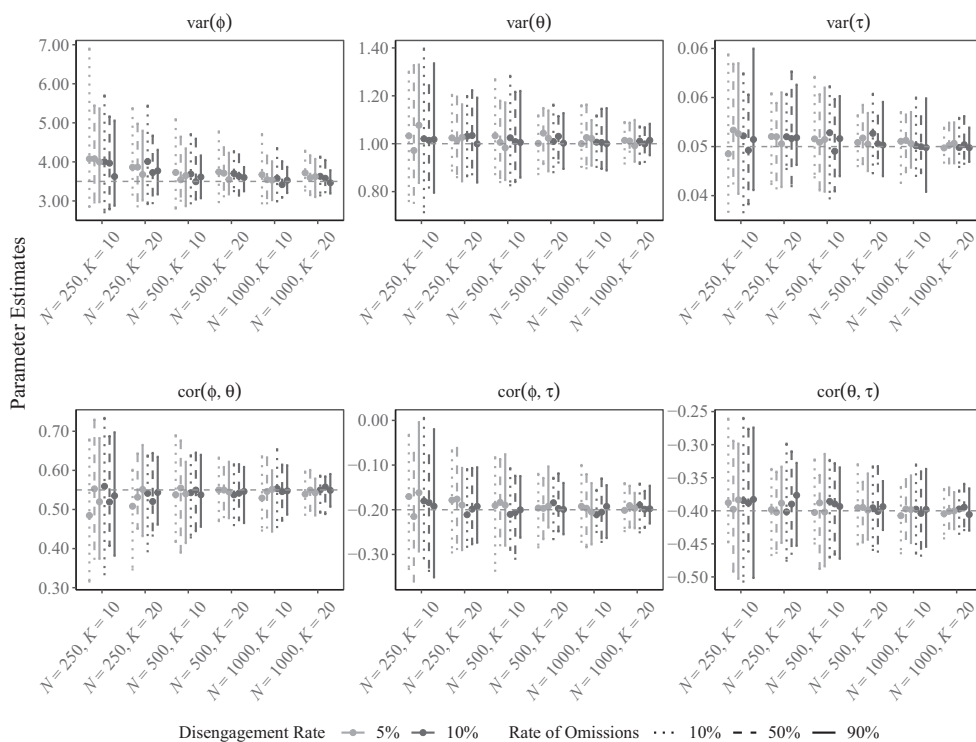
Figure 2. Medians and 50% ranges of person parameter variance and correlation estimates. The dashed horizontal line indicates the respective true parameter. Note that y -axes differ in scale. \phi = engagement; \theta = ability; \tau = speed; N = number of examinees; K = number of items. The shades of the lines denote the rates of disengaged behaviour. The percentages of omissions on disengaged behaviour are given by different line types.
