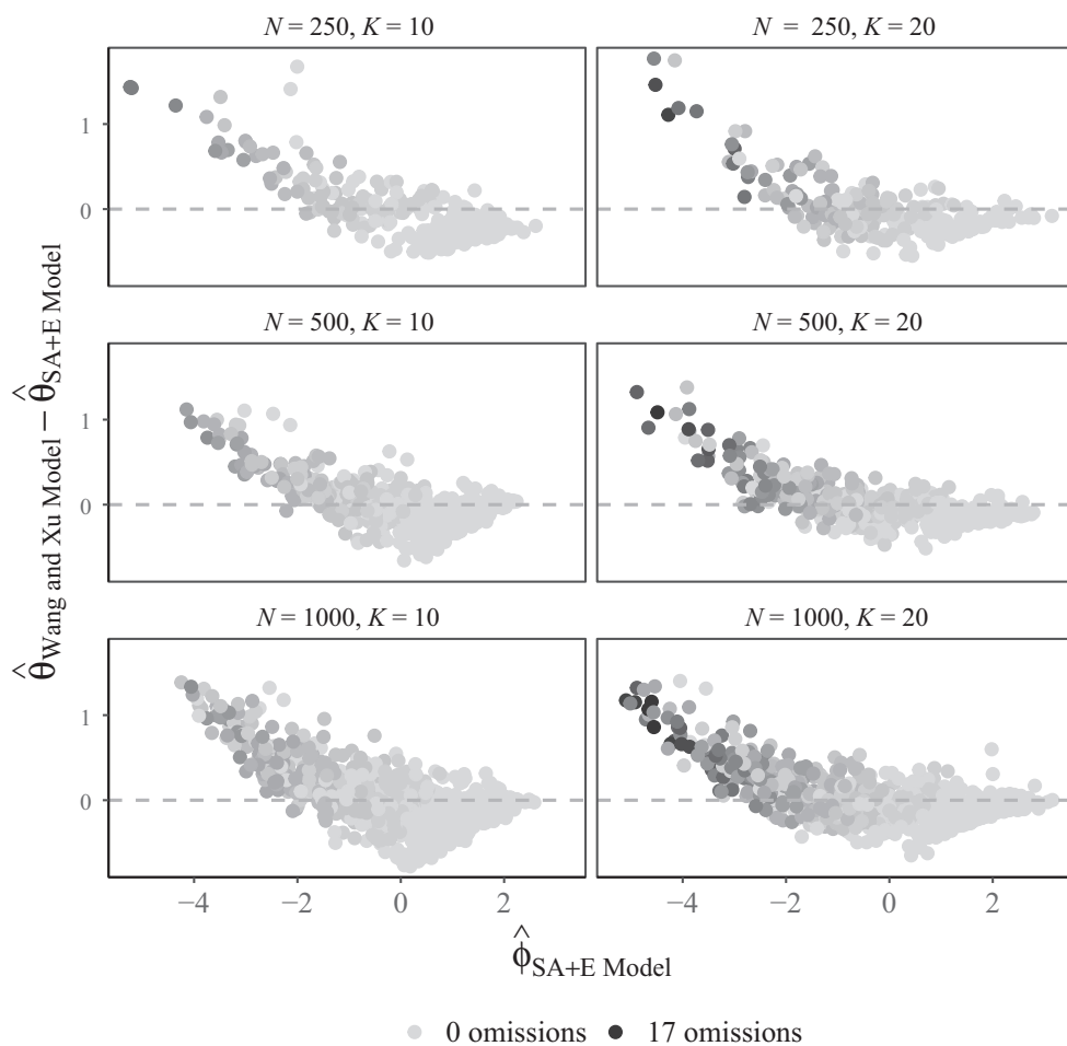
Figure 9. Differences in ability estimates retrieved from the Wang and Xu model and the SA+E model plotted against engagement estimates retrieved from the SA+E model. The colour of the points denotes the number of item omissions for each examinee, with darker shades indicating a higher number of item omissions. N = number of examinees; K = number of items.
