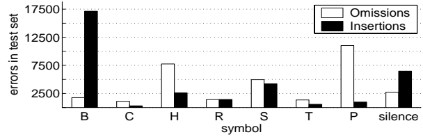
Fig. 3. Omission and insertion errors for each symbol.
