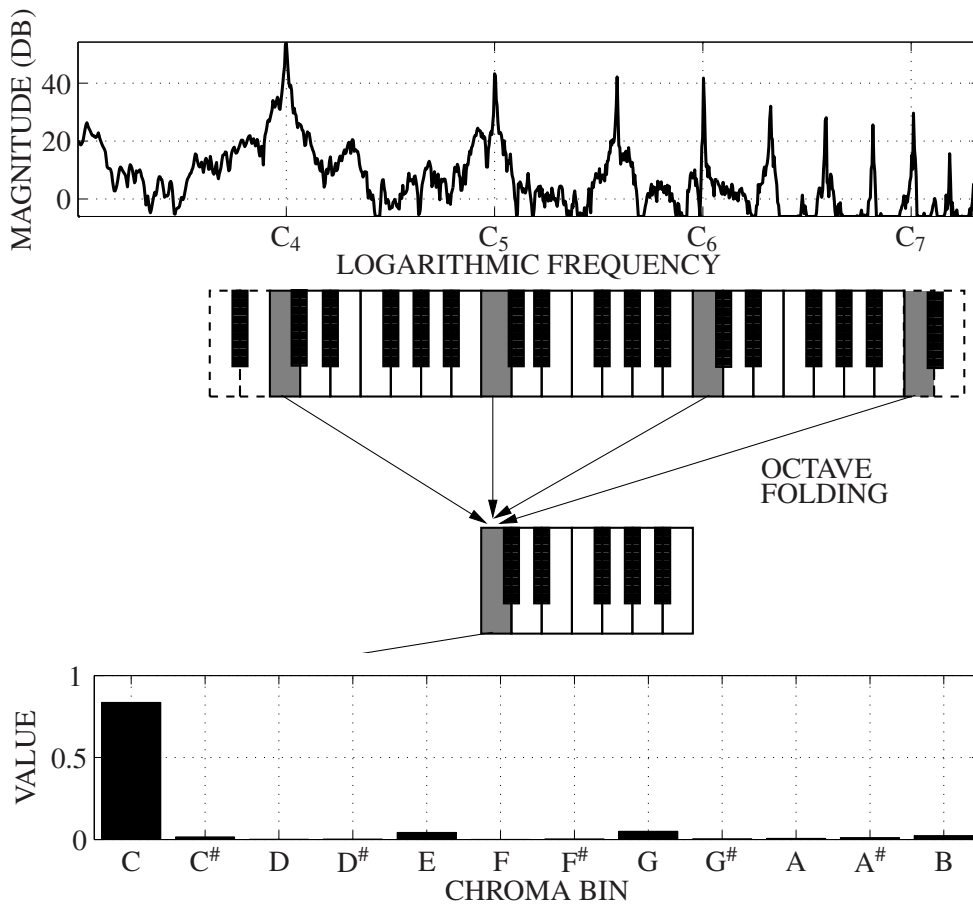
Figure 3.5: Illustration of the chroma calculation with octave folding from an input signal containing a single piano note C_4 . Top panel contains the magnitude spectrum, and the remaining panels illustrate how the energy corresponding to all occurrences of chroma “C” are gathered through octave folding to the single chroma vector bin.
