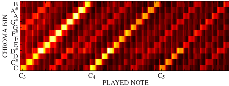
Figure 3.6: An example of a chroma feature matrix calculated from an input signal of an ascending scale of three octaves from C_3 to B_5 played with a MIDI piano. The brighter the image element, the larger the value in the chroma matrix.
