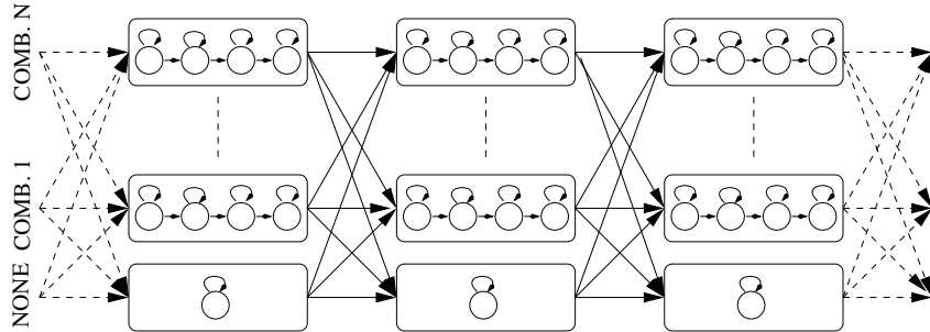
Figure 2: Illustration of the basic idea of drum transcription with connected HMMs for drum combinations. The decoding aims to find the optimal path through the models given the observed acoustic information.
