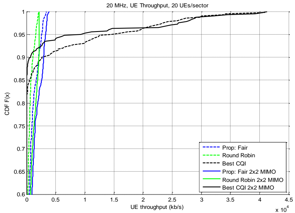
Figure 5.12: UE throughput plots for PF, RR and BCQI with 2X2 MIMO.
