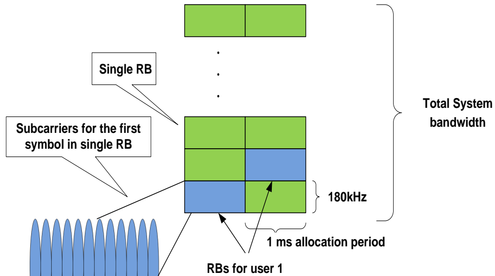
Figure 4.2: OFDMA resource allocation in LTE. [12]
