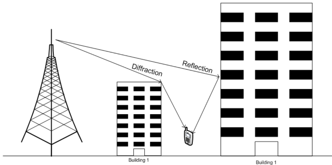
Figure 2.3: Multipath propagation
