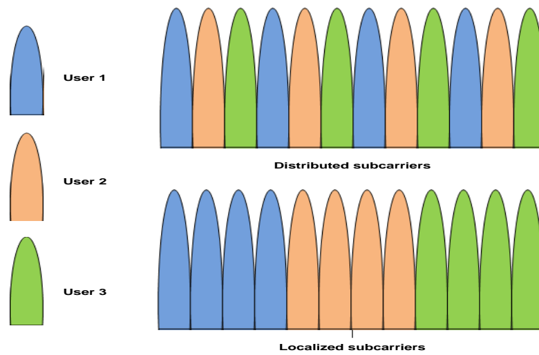
Figure 4.4: Subcarrier allocation for multiple users in SC-FDMA.
