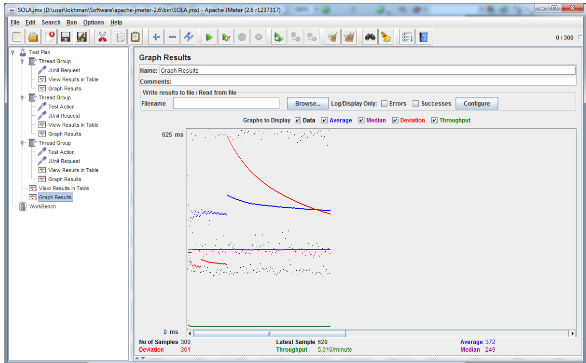
Figure 4.6 General Test of 1 hr with 12 seconds pause using JMeter
