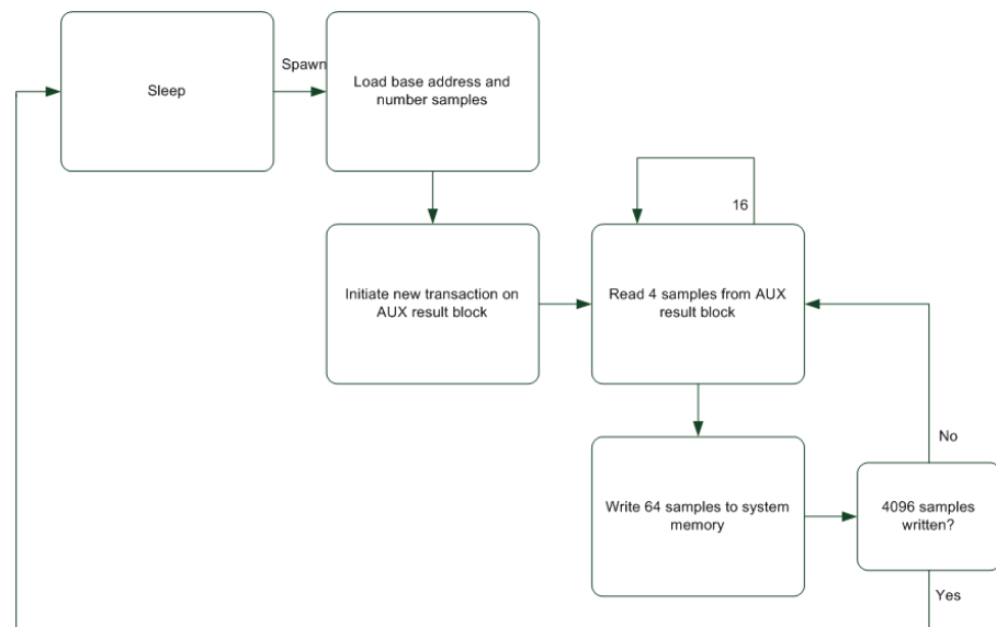
Figure 5.16. Storing thread operation.
