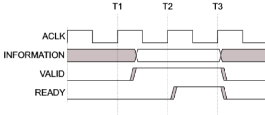
Figure 4.4. AMBA handshaking [12].
