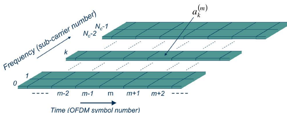
Figure 2.7. OFDM time-frequency grid [8, Fig.3.4].
