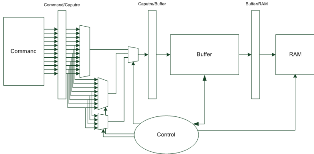
Figure 5.5. Command block datapath.
