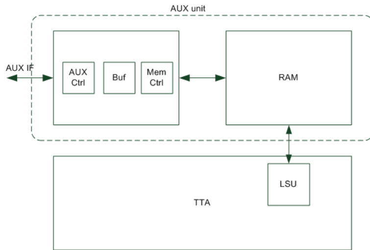
Figure 4.9. Auxiliary unit.
