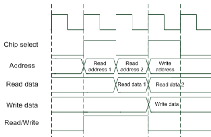
Figure 4.3. RAM timing.
