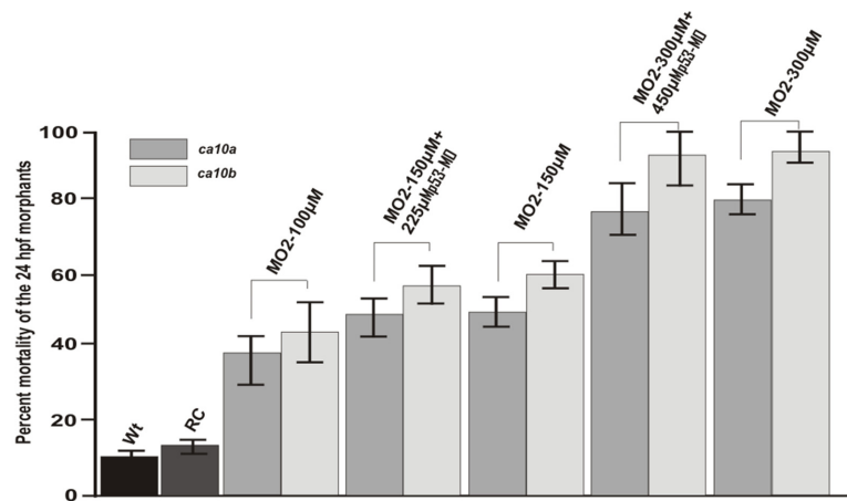
Fig 9. The percent mortality of the morphant larvae at 24 hpf. The mortality rate of ca10a and ca10b MO injected larvae was significantly higher than that of controls ( P < 0.001 ). Larvae injected with p53 -MOs along with ca10a or ca10b -MOs and larvae injected with ca10a or ca10b -MOs alone did not show significantly different mortality rates.
