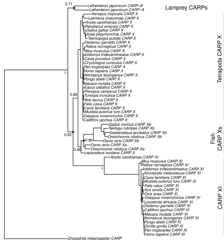
Fig 1. Bayesian phylogenetic tree of CARP sequences. Numbers at the nodes indicate posterior probabilities, and branch lengths are proportional to distances. A table of full details of the sequences is given as S1 Table .
