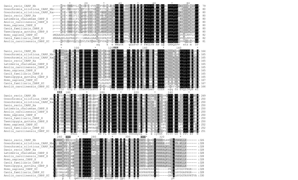
Fig 2. Multiple sequence alignment of selected CARP X-like protein sequences. Groups of three asterisks (***) above the sequences indicate conserved N-glycosylation motifs in all CARP X-like proteins, and letters 'xxx' above the sequences indicate N-glycosylation motifs which are only found in either CARP X or CARP XI sequences (NFS and NIT, respectively).
