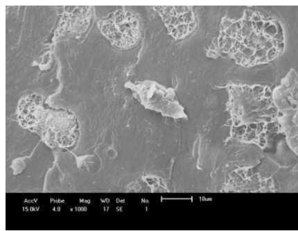
PET-PC-PEAD 1000X
