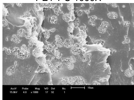
PET-PC-PEAD-COMP 1000X
