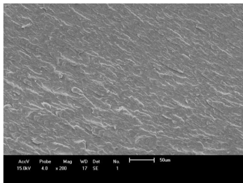
PET-PC 200X
