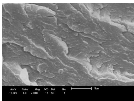
PET-PC 3000X
