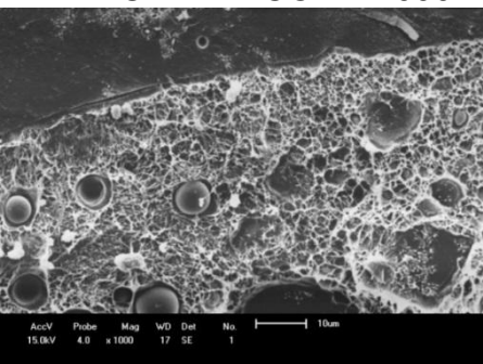
PET-PC-PEAD-EXT3 1000X
