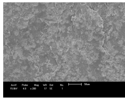
PET-PC-PEAD-COMP-EXT1,5 200X
