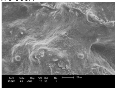
PET-PC-PEAD-COMP-EXT3 500X
