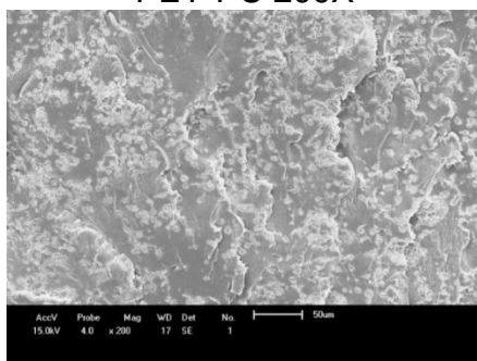
PET-PC-PEAD-COMP 200X
