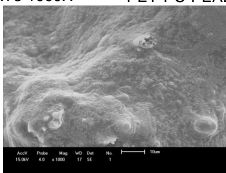
PET-PC-PEAD-COMP-EXT3 1000X
