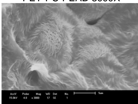
PET-PC-PEAD-EXT1,5 3000X
