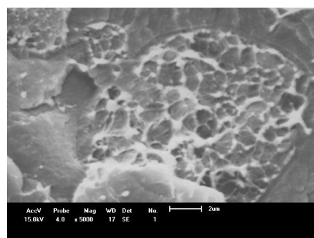
PET-PC-PEAD-COMP-EXT1,5 5000X
