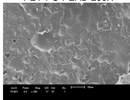
PET-PC-PEAD-EXT1,5 200X
