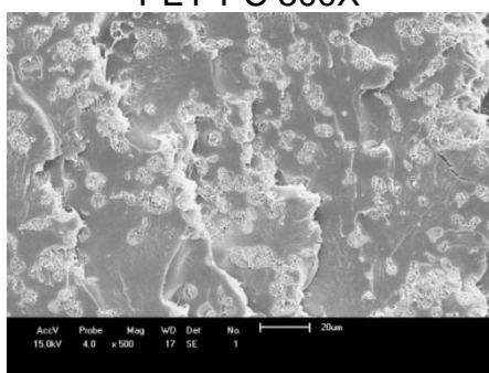
PET-PC-PEAD-COMP 500X
