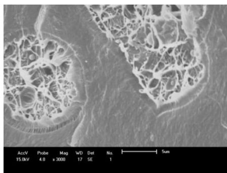
PET-PC-PEAD 3000X
