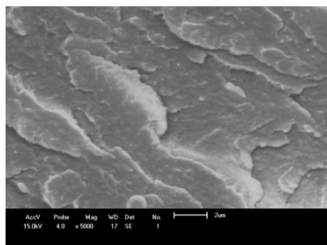
PET-PC 5000X
