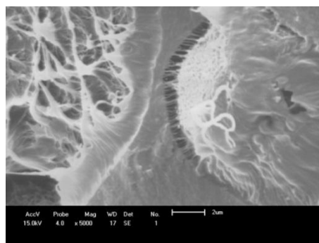
PET-PC-PEAD 5000X
