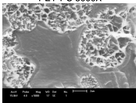
PET-PC-PEAD-COMP 5000X
