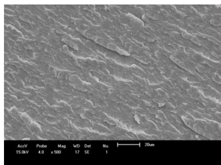
PET-PC 500X
