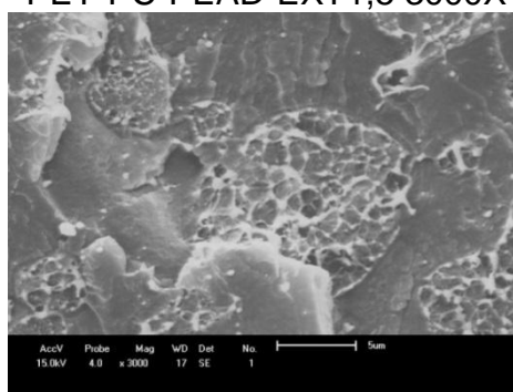
PET-PC-PEAD-COMP-EXT1,5 3000X
