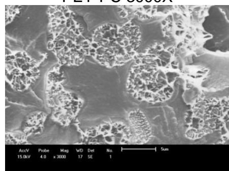
PET-PC-PEAD-COMP 3000X
