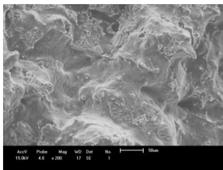
PET-PC-PEAD-COMP-EXT3 200X
