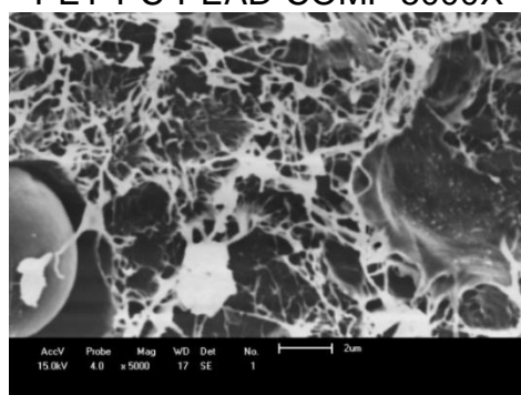
PET-PC-PEAD-EXT3 5000X
