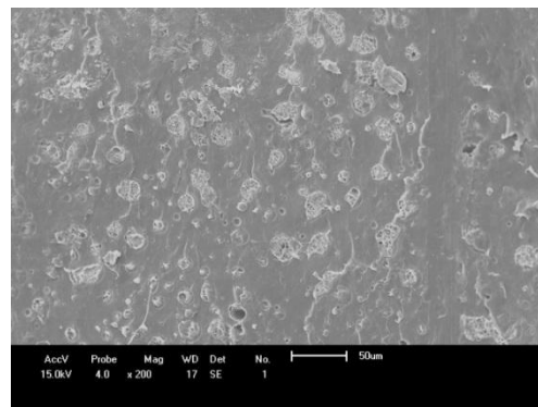
PET-PC-PEAD 200X
