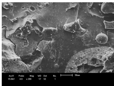
PET-PC-PEAD-EXT3 200X
