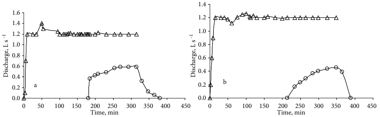
Figure 3. Typical inflow ( \Delta ) and outflow (o) hydrographs for EFO third event (a) and AFO second event (b) in 1993.
