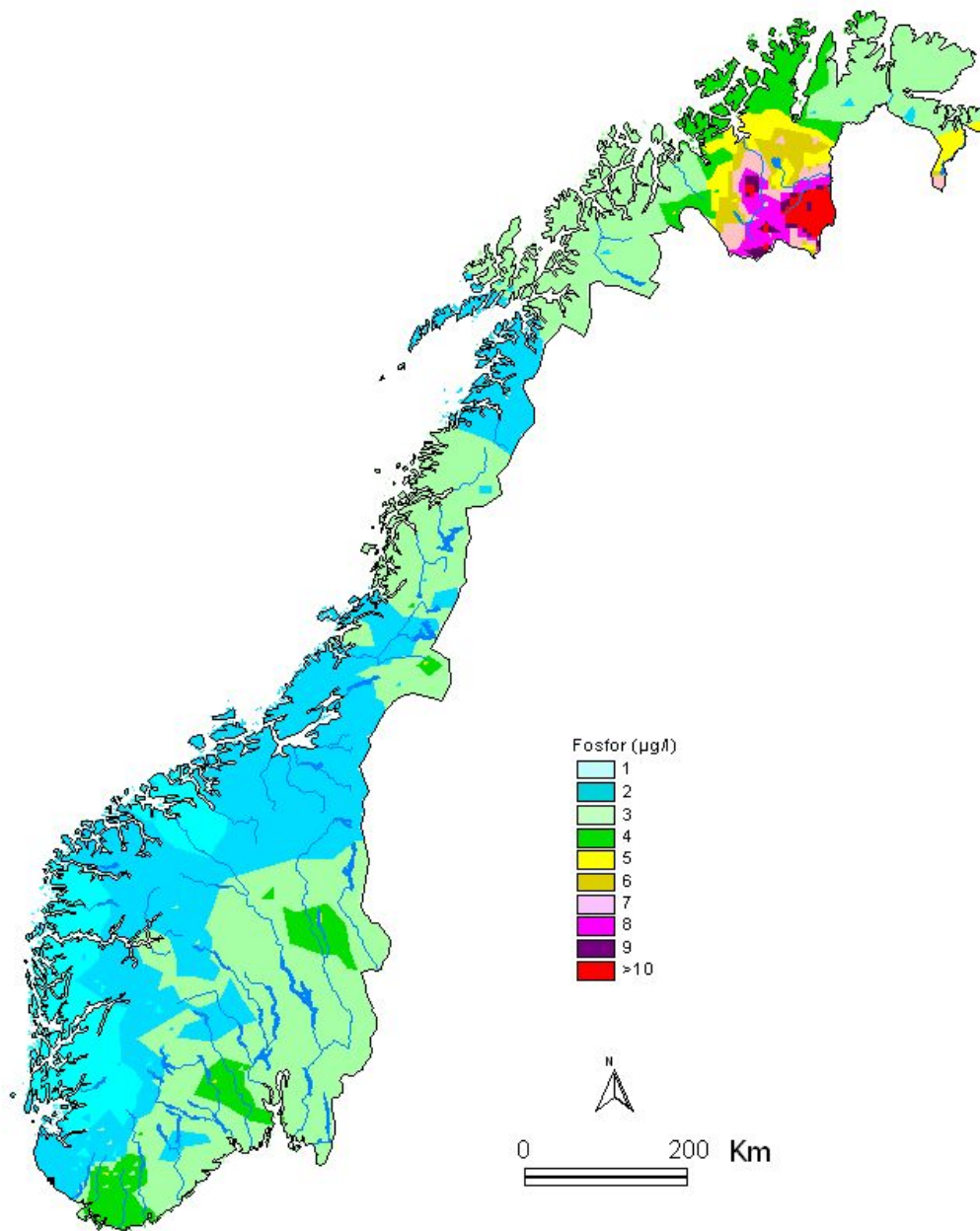
Figure 40: Phosphorus concentrations in mountainous areas produced by using GIS.
