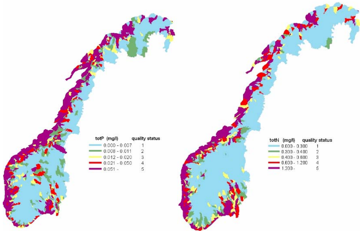
Figure 25. Phosphorus (left) and nitrogen concentrations in 2004, calculated by the TEOTIL model
