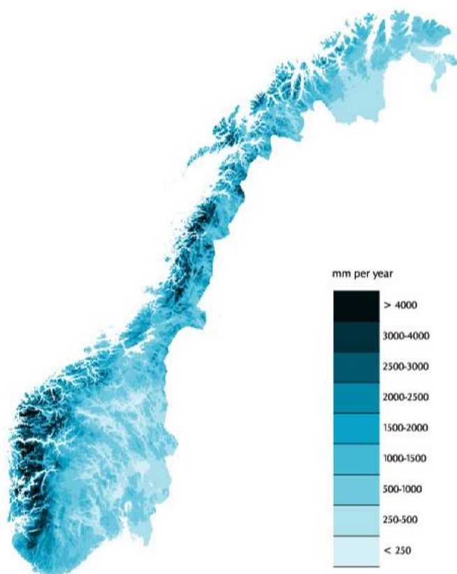
Figure 7: Annual average runoff (mm/year) for Norway for the period 1961-1990.
