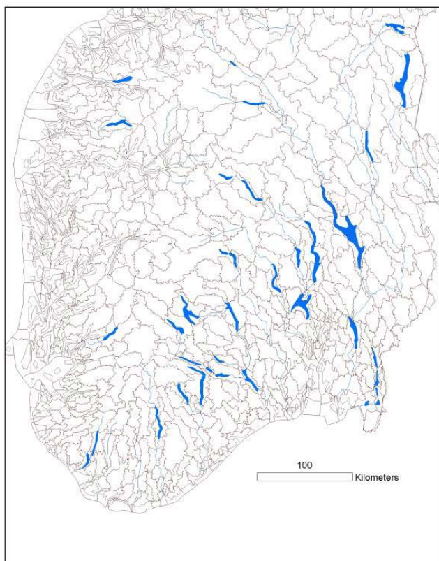
Figure 24. Statistical areas in the southern part of Norway
