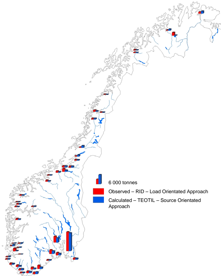
Figure 10. Comparison between observed and estimated nitrogen load in the rivers monitored in the RID Programme in 2004
