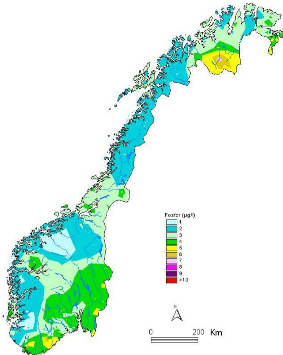
Figure 41. Phosphorus concentrations in forested areas produced by GIS
