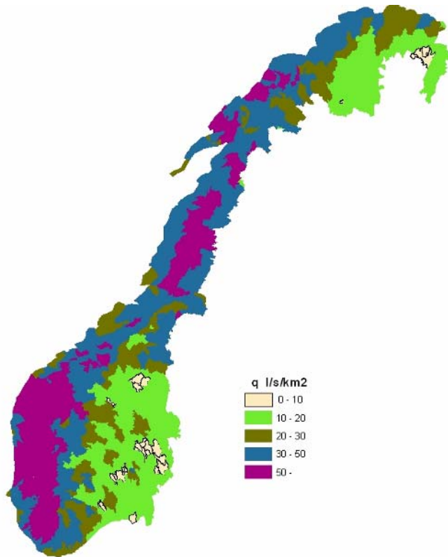
Figure 20. Discharge flow in liter per second and km 2 in Norway in 2004
