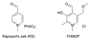
Fig. 70 PLP-analogues used as transamination agents: Rapoport's salt 619 and FHMDP. 621
