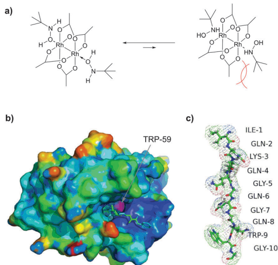
Fig. 45 Optimised metallocarbenoids-based approach, described by Francis and collaborators. 452 (a) Proposed binding of \text{tBuNH}_2\text{OH} with \text{Rh}_2(\text{OAc})_4 at pH 6.0. \text{O} -Coordination is favoured due to a lower steric hindrance of tert -butyl groups with acetate ligands. (b) Crystal structure of wild type FKBP (pdb: 1A7X), containing a single, buried tryptophan residue TRP-59 (shown in magenta), which is unavailable for modification under non-denaturing conditions. (c) A peptide tag (IQKQGQGWG) incorporated into fusion FKBP protein expressed in E. coli as C-terminal intein fusion. The total level of modification was estimated to be in excess of 40%.
