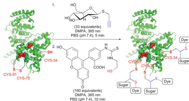
Fig. 28 Glycosylation and fluorescent labelling of bovine serum albumin (BSA, pdb: 3V03) by TEC (first step) followed by TYC (second step) with 2,2-dimethoxy-2-phenylacetophenone (DMPA) as a photoinitiator. 345
