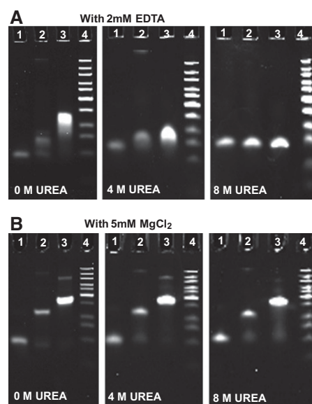
FIGURE 3. Effect of magnesium ions on the resistance of pRNA 3WJ to urea denaturation, assayed by 15% PAGE gels with (A) 2 mM EDTA and (B) 5 mM MgCl_2 . (Lane 1) Single RNA oligo b_{3wj} ; (lane 2) sample annealed from two oligos a_{3wj} and b_{3wj} ; (lane 3) 3WJ assembled from three oligos a_{3wj} , b_{3wj} , and c_{3wj} ; and (lane 4) DNA ladder.
