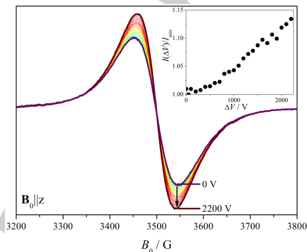
Figure 3. X-band EPR single-crystal data of 1 at \mathbf{B}_0 || \mathbf{z} under varying electric fields. Experimental conditions: f = 9.80 GHz, mod. ampl. = 10 G pp , power: 2 mW. The inset shows the electric field dependence of the integrated intensities of the experimental spectra ( I_{\min} = 1 ).
