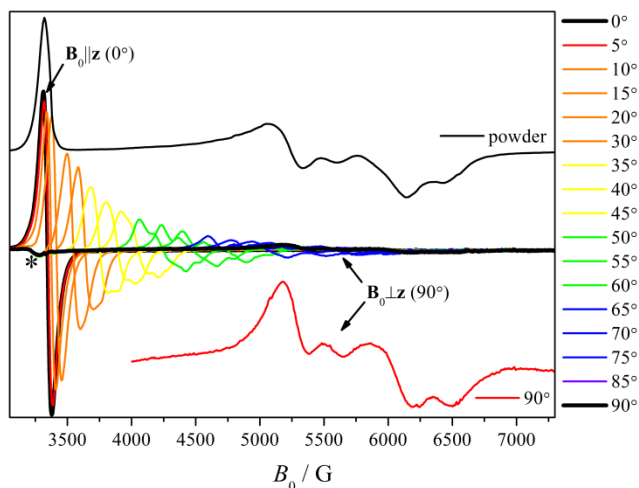
Figure 2. X-band EPR single-crystal and powder data of 1 at 4.2 K. The asterisk at ~3300 G indicates a cavity impurity. Experimental conditions: f = 9.31 GHz, mod. ampl. = 10 G pp . Single-crystal spectra (0-90°): Power = 2.5 mW. Single-crystal spectrum at 90° (red line): Power = 10 mW. Powder spectrum (black line): Power = 0.02 mW.
