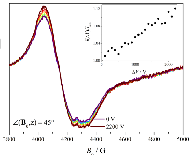
Figure 4. X-band EPR single crystal data of 1 at \angle(\mathbf{B}_0, \mathbf{z}) = \pi/4 under varying electric fields. Experimental conditions: f = 9.80 GHz, mod. ampl. = 10 G pp , power: 4 mW. The inset shows the electric field dependence of the integrated intensities of the experimental spectra ( I_{\min} = 1 ).
