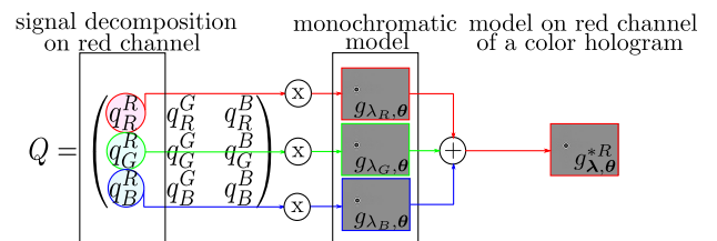
Fig. 6. Principle of crosstalk correction.
