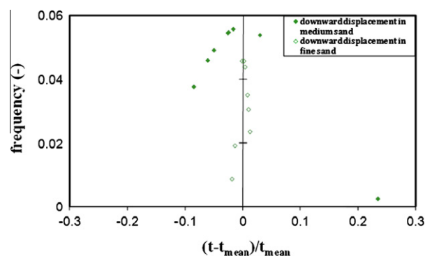
Fig. 7. Measured dimensionless arrival times of the water/DNAPL front in both medium sand and fine sand: case of vertical-downward water displacement at low DNAPL injection flow rate (40 mL/min).
