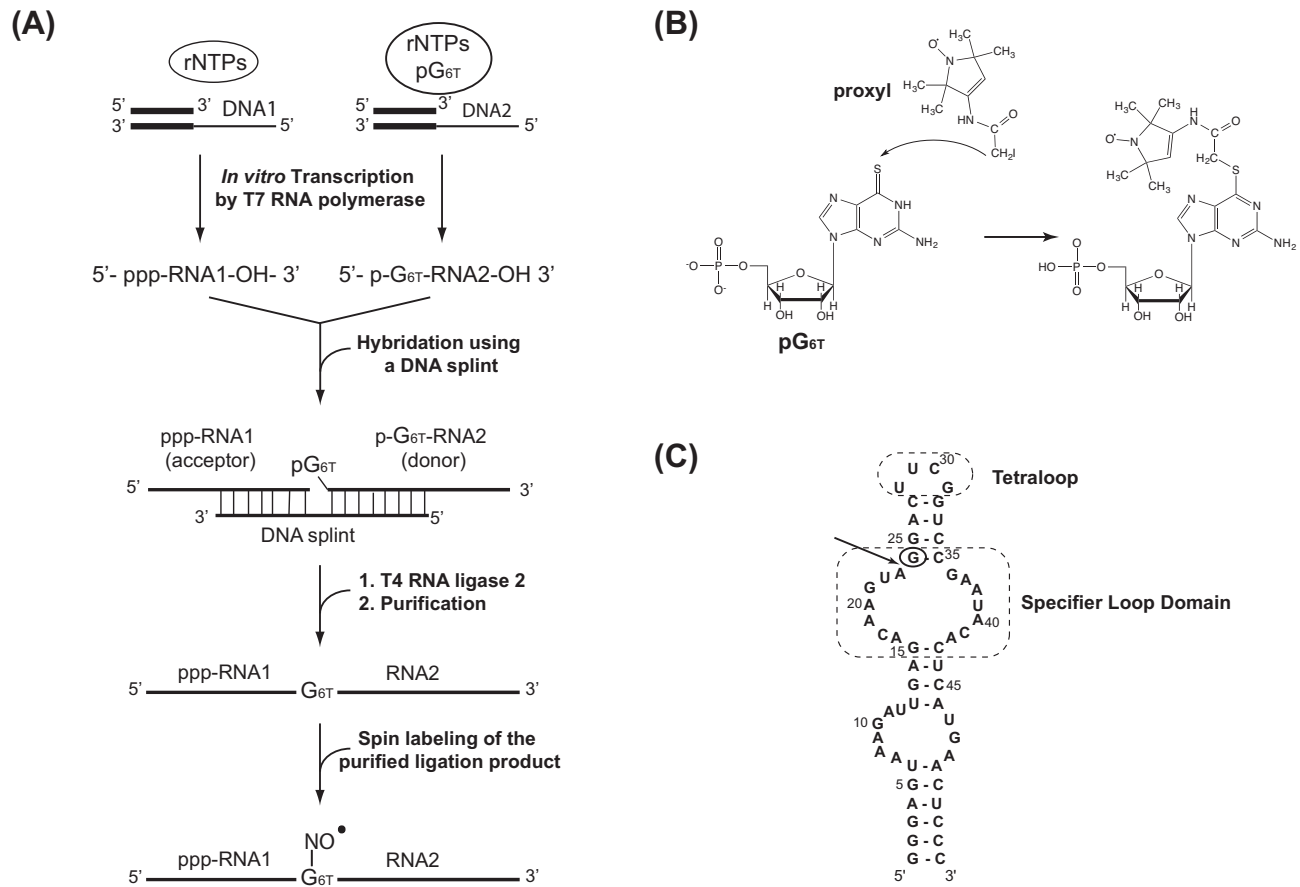
Figure 1. Method for the site-directed spin labeling approach. (A) Schematic representation of the synthesis of site-specific spin labeled RNA. 6-thioguanosine-5'-O-monophosphate (pG 6T = 6-T-GMP) is incorporated at a specific position. (B) The proxyl-RNA coupling reaction involves the addition of 3-(2-Iodoacetamido)-proxyl on 6-thioguanosine-5'-O-monophosphate. (C) Secondary structure of the 55-nt (tyrS) RNA molecule corresponding to the specifier loop domain and K-turn sequence motif of the tyrS leader RNA. The Specifier Loop Domain and the tetraloop are boxed. The arrow indicates the chosen segmentation site and the circle indicates the thio-modified site.
