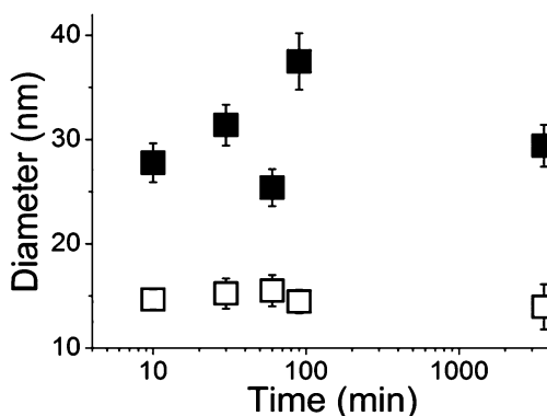
Fig. 3 Evolution of the size distribution of NP@ 94 (■) and NP@ 94 diluted (□) in sodium chloride medium (0.15 M NaCl) after 24 h. 22c
