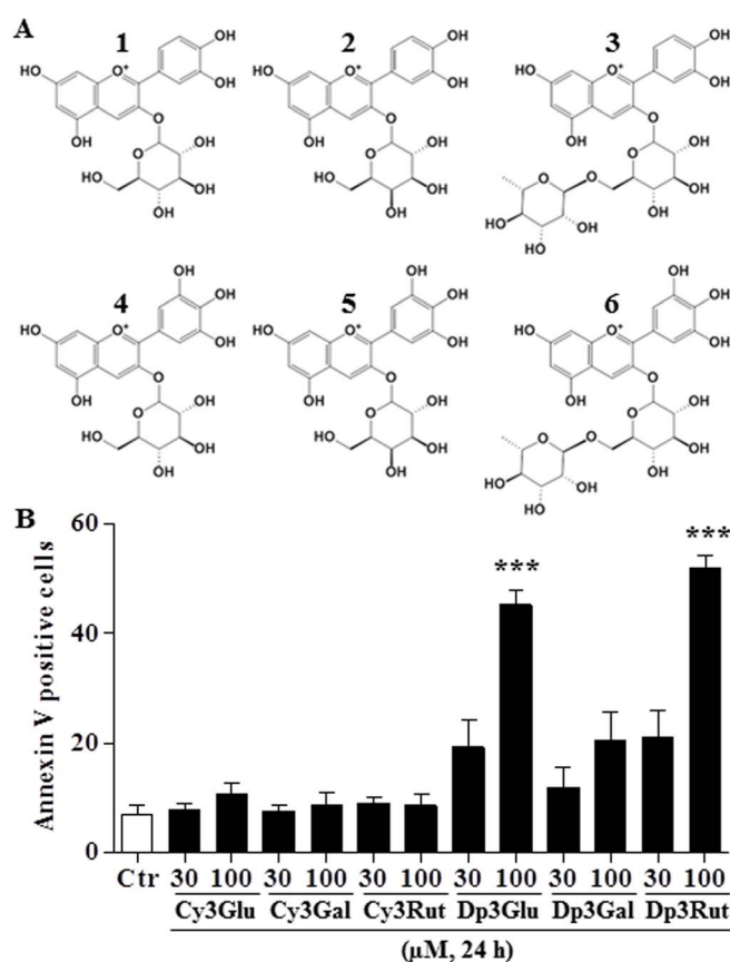
Figure 2 | Chemical structures of anthocyanins present in Antho 50 (A): cyanidin-3- O -glucoside (1), cyanidin-3- O -galactoside (2), cyanidin-3- O -rutinoside (3), delphinidin-3- O -glucoside (4), delphinidin-3- O -galactoside (5) and delphinidin-3- O -rutinoside (6). B CLL cells were exposed to 30 or 100 \mu\text{M} of the indicated anthocyanin for 24 h. Then apoptosis rate was determined by flow cytometry using annexin V-FITC/PI assay (B). The control (Ctr) represents untreated cells. The data are representative of cells from four CLL patients. Values are shown as means \pm S.E.M. (n = 4); ***, P < 0.001 versus control.
