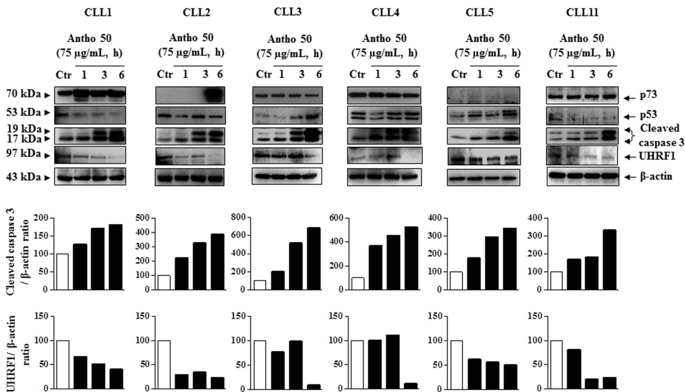
Figure 3 | Antho 50 induces caspase 3 activation and UHRF1 down-regulation independently of p53 and p73. B CLL cells were incubated with Antho 50 at 75 \mu g/mL for the indicated times and thereafter the expression of the p53, p73, cleaved caspase 3 and UHRF1 was studied using Western blot. The control (Ctr) represents untreated cells harvested at 6 h. The data are representative of cells from six CLL patients. Cleaved caspase 3 and UHRF1 expression levels were analyzed by densitometry and represented as percentage compared with control.
