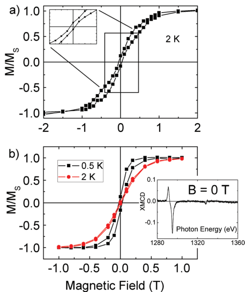
Fig. 2 Field-dependent magnetization measured at the maximum of (a) the Tb M_5 edge XMCD at T = 2 K and (b) the Dy M_5 XMCD edge at T = 0.5 K (black) and T = 2 K (red), normalized to the saturation magnetization.
