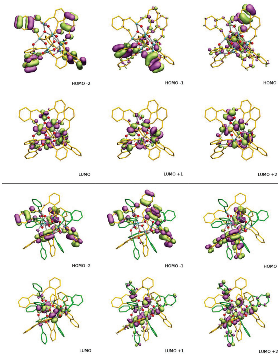
Fig. 9 \text{Ti}_{10}\text{O}_{12}(\text{cat})_8 (top) and \text{Ti}_{10}\text{O}_{12}(\text{cat})_8(\text{py})_8 (bottom): representation of the HOMO, HOMO–1 and HOMO–2 as well as the LUMO, LUMO+1 and LUMO+2 orbitals for both complexes. Catecholato ligands are represented in yellow, and pyridine ligands in green. Hydrogen atoms are omitted for clarity.
