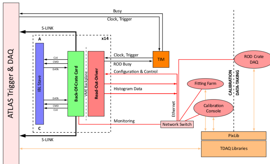
Figure 50. Schematic of the IBL read-out system.
