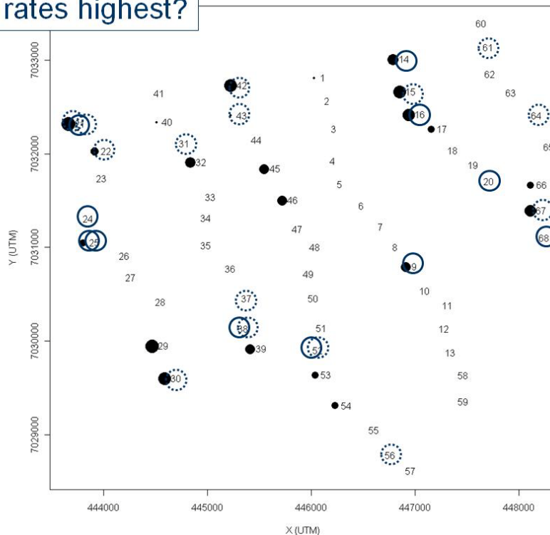
Figure 27. Spatial representation of the relative (log-transformed) 3D collision risk rates per wind turbine within the Smøla wind-power plant in Central Norway. The numbers depict the turbine numbers while the size of the black dots indicate the risk (no dot equals no risk, while larger dots indicate increased risk). Turbine numbers with solid and dotted circles indicate recorded sub-adult and adult collision victims, respectively (each circle indicates one victim).
