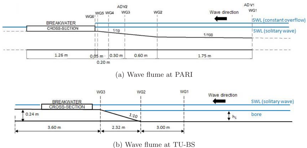
Fig. 4. Experimental setups and measuring devices in the wave flumes at: (a) PARI ( 105 \text{ m} \times 0.78 \text{ m} \times 2.5 \text{ m} ) [Guler et al. , 2015], and (b) TU-BS ( 90 \text{ m} \times 2.0 \text{ m} \times 1.2 \text{ m} ) [LWI, 2015a]. Locations of instruments over the breakwater regions are shown in Figs. 5(a)–7. Not to scale.
