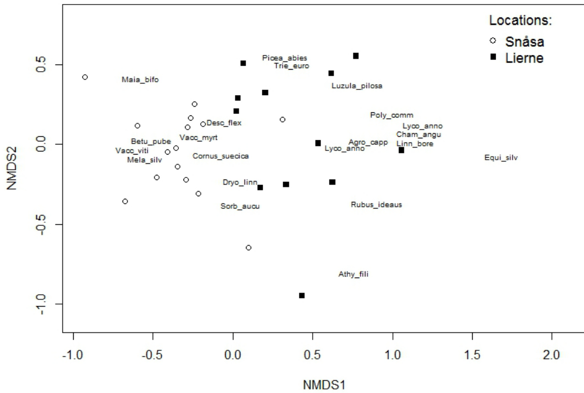
Figure 1. Ordination plot for 2008 showing species and plots present in an ecological space. Plots represent all species present, and their percent canopy cover.
