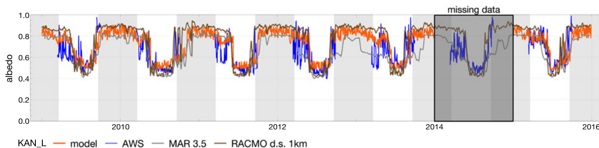
Fig. 7. Simulated and observed albedo at KAN_L with the model parameters from the optimisation at KAN_M and KAN_U and the englacial concentration of BC of 1 and 200 \text{ ng g}^{-1} dust.
