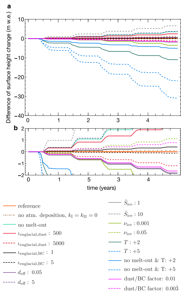
Fig. 9. Simulations of surface height change relative to the optimised settings at KAN_M2010 (orange) in (a). Panel (b) shows a zoom in on (a).
