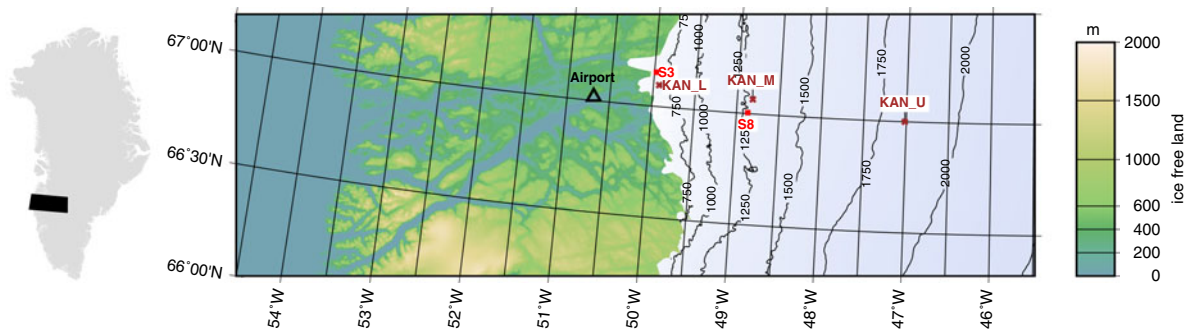
Fig. 1. Weather stations and sampling sites at the K-transect in western Greenland, near the Kangerlussuaq airport (topography data by Morlighem and others (2014)). Brown crosses mark the PROMICE weather stations operated by GEUS. Red squares mark additional mass-balance sites where ice samples have been taken close to the PROMICE stations (Wientjes and others, 2012). Station KAN_U (1840 m a.s.l.) is located near the equilibrium line. Locations S8 and KAN_M (1270 m a.s.l.) are located in the 'dark region' with a lower albedo.
