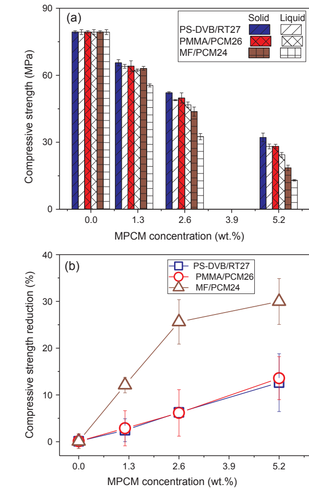
Fig. 13. (a) The compressive strength of GPC containing microcapsules below (20 °C) and above (40 °C) the melting range of PCM and (b) the compressive strength reduction between the solid and liquid state of PCM.
