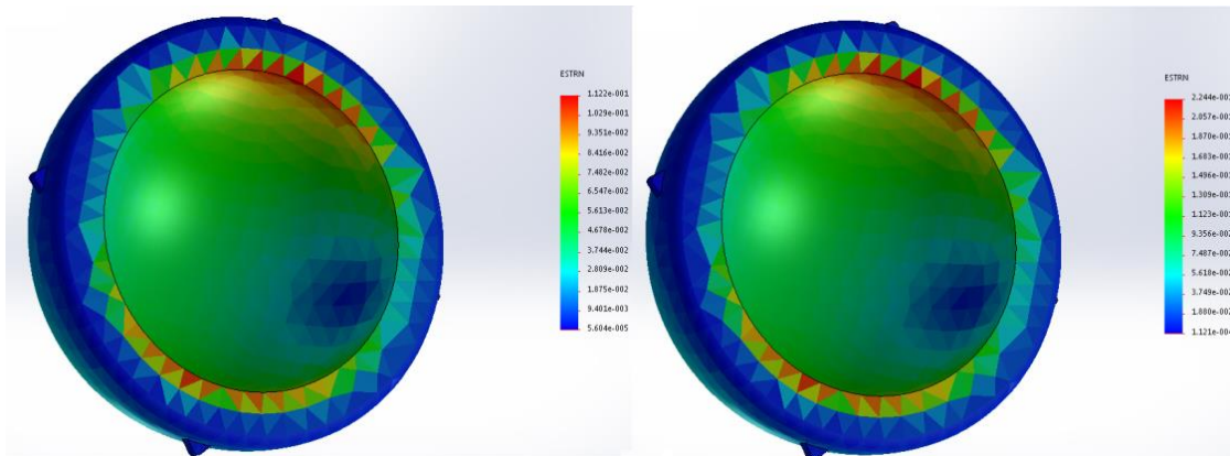
Fig. 4. Deformations in polyethylene socket inlay for 100 (left) and 200%BW (right)
