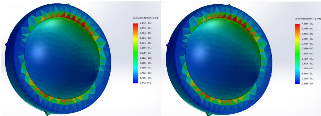
Fig. 3. Stress distribution in ceramic socket inlays for 100 (left) and 200%BW (right)
