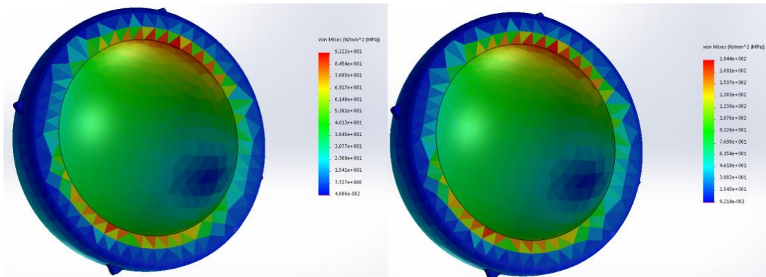
Fig. 2. Stress distribution in polyethylene socket inlays for 100 (left) and 200%BW (right)
