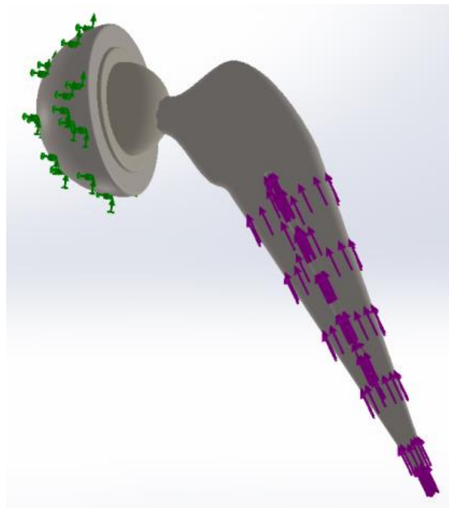
Fig. 1. Places of fixing the model and application of the force
