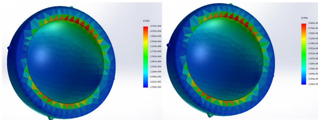
Fig. 5. Deformations in ceramic socket inlay for 100 (left) and 200%BW (right)
