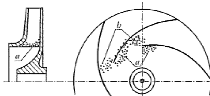
Fig. 1. Damage due to cavitation in the impeller of a centrifugal pump [2], [6]
