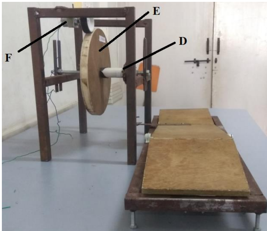
Fig. 4 Cross sectional view of the prototype where D - spur Gear, E - fly wheel, F - gear wheel motor
