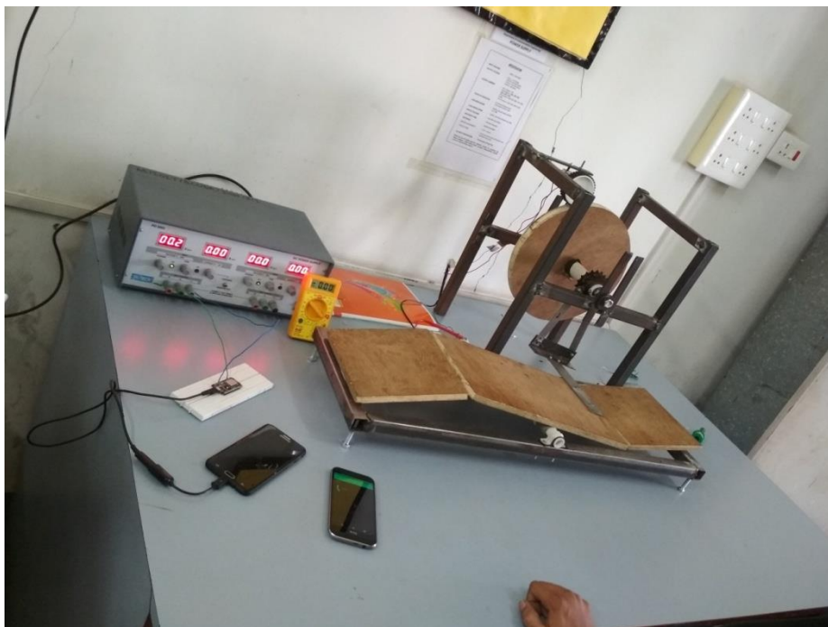
Fig. 5 IOT based Measurement
