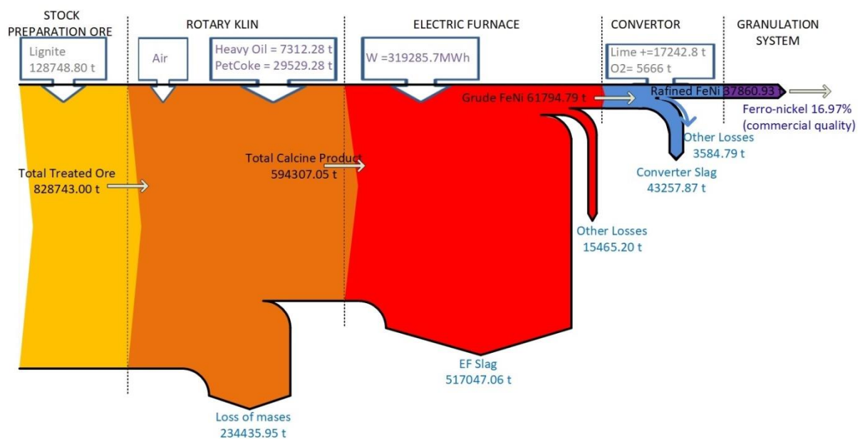
Fig. 5. The diagram of material balance of the process of the Fe-Ni production in 2017.
