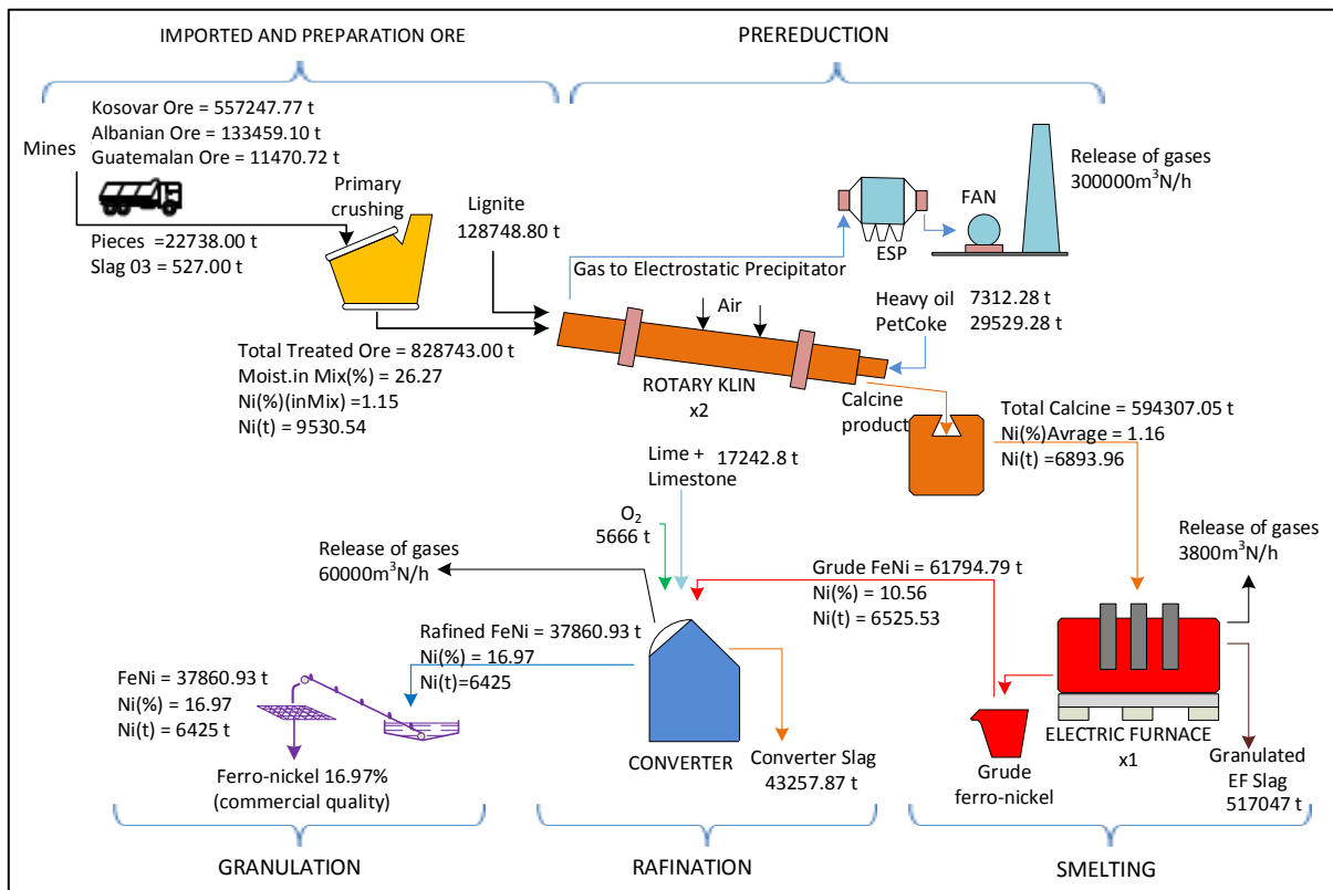
Fig. 4. Schematic representation of the Fe-Ni production process in the new foundry of new Ferronickel in Drenas - Material balance sheet of the used and planned amount in 2017 [1,6,9].
