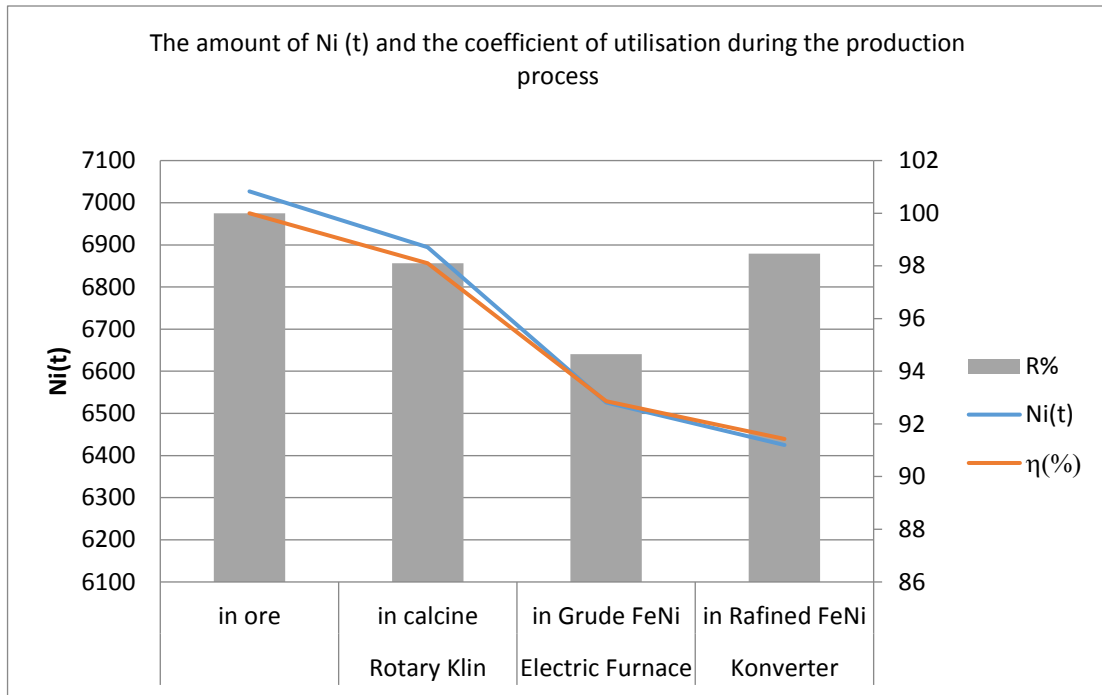
Fig. 3. Graphic representation of Ni (t), coefficient of Fe-Ni (η) ore utilisation, the coefficient of utilisation at certain stages of the process (R).
