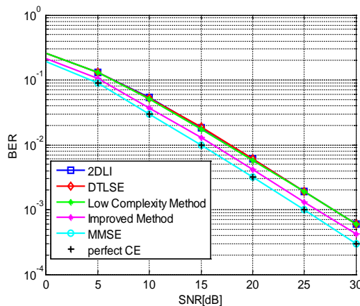
Figure 3: BER vs. SNR for the first, second proposed and other methods under TU-6 channel for 50-Hz Doppler frequency shift.
