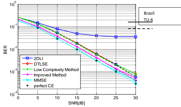
Figure 6: BER vs. SNR for the proposed low complexity, improved methods and other methods under 300-Hz Brazil-D and 50-Hz TU-6 channel.
