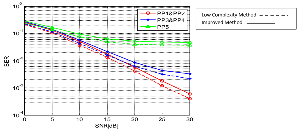
Figure 10: BER vs. SNR of the proposed low complexity, improved methods for considered pilot patterns under TU-6 channel.
