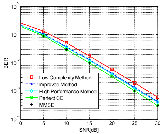
Figure 7: BER vs. SNR for the proposed high performance method and other methods under TU-6 Channel
