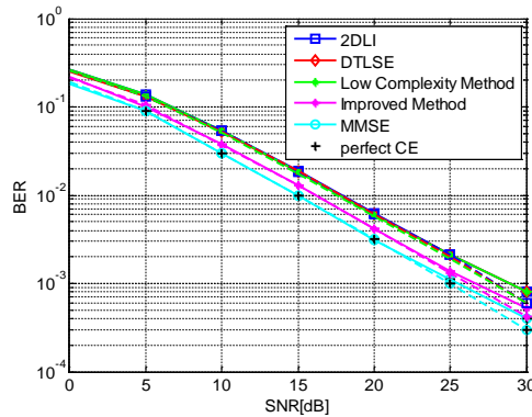
Figure 4: BER vs. SNR for the proposed low complexity, improved methods and other methods under TU-6 channel for 300-Hz Doppler frequency shift.
