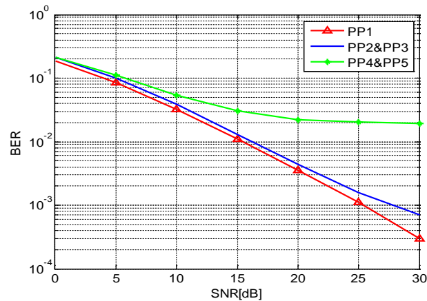
Figure 11: BER vs. SNR of the proposed high performance method for considered pilot patterns under TU-6 channel.
