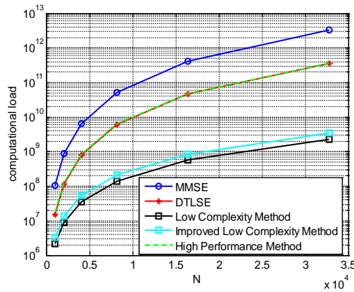
Figure 2: The computational load for the considered methods.
