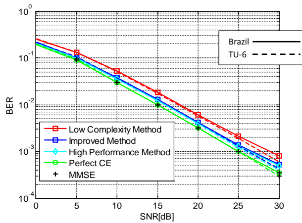
Figure 8: BER vs. SNR for the proposed high performance method and other methods under Brazil-D channel and TU-6 Channel
