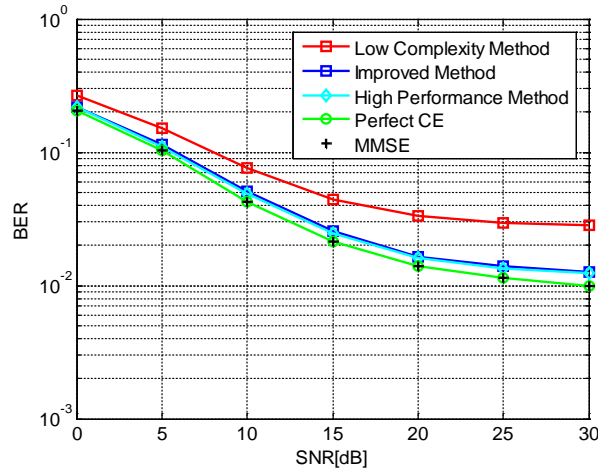
Figure 9: BER vs. SNR for the proposed high performance method and other methods under high delay Rayleigh fading Channel
