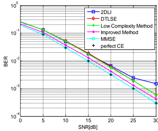
Figure 4: BER vs. SNR for the proposed low complexity, improved methods and other methods under TU-6 channel for 300-Hz Doppler frequency shift.
