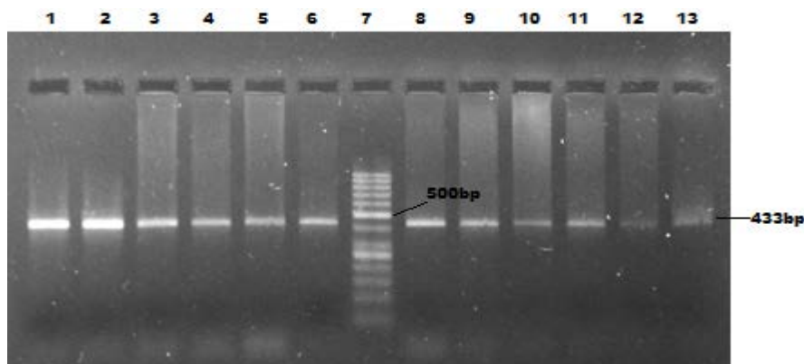
Fig 1. Agarose gel electrophoresis of amplified apo-A1 gene region. All lanes contain a 433bp amplified product, except lane 7 which contains 500bp DNA ladder.
