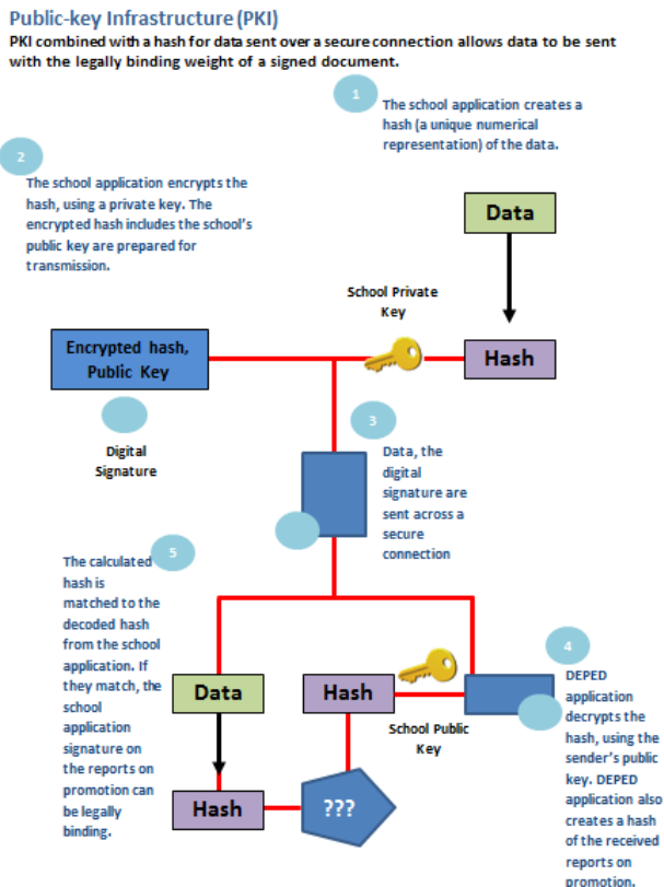
Figs. 4. PKI infrastructure
