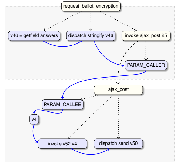
Figure 3: Relevant parts of a backwards slice with XMLHttpRequest.send() as the seed.
