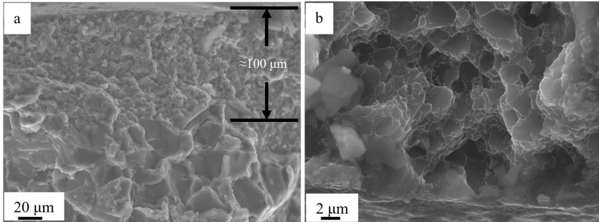
Figure 4. The structure of the destruction surface of the hypereutectic silumin subjected to an intense pulsed electron beam ( 35 \text{ J / cm}^2 ; 200 \text{ } \mu\text{s} , 20 pulses 0.3 \text{ s}^{-1} ).
