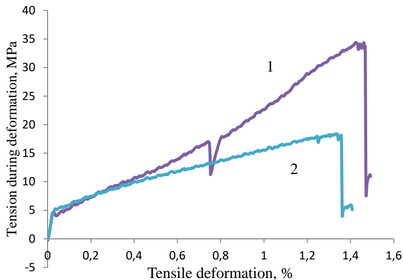
Figure 2. Deformation curves of the hypereutectic silumin subjected to electron beam irradiation ( 200 \mu\text{s} , 20 \text{ imp. } 0.3 \text{ s}^{-1} ): curve 1 - 35 \text{ J / cm}^2 ; curve 2 is 15 \text{ J / cm}^2 .
