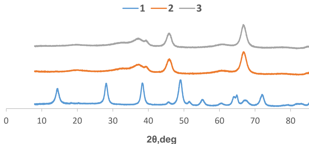
Figure 4. X-ray diffraction patterns of samples. 1 - initial pseudo-boehmite; 2 - aluminium oxide; 3 - catalytic system.
