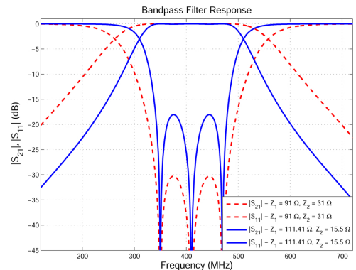
Fig. 2. Simulation results for the bandpass filter with two different equivalent impedance ratios. The obtained 3 dB bandwidth is 48.8%, which exceeds the original requirement, however was this not weighted so high. The main focus has been the combination of the notch and bandpass filter.
