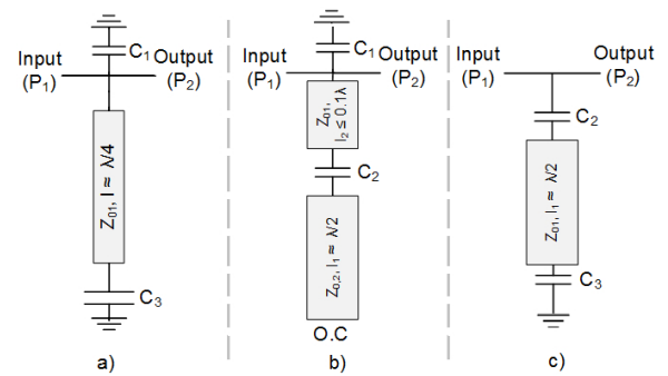
Fig. 3. Three different notch configurations. a) Tunable parallel resonator, b) Capacitive coupled series resonator c) Capacitive coupled tunable series resonator.
