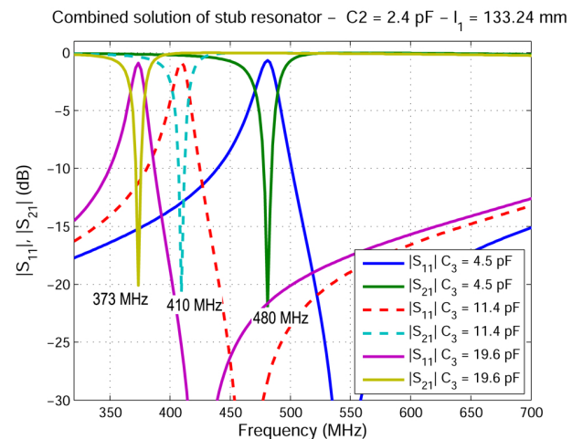
Fig. 4. Simulated response of the notch filter.
