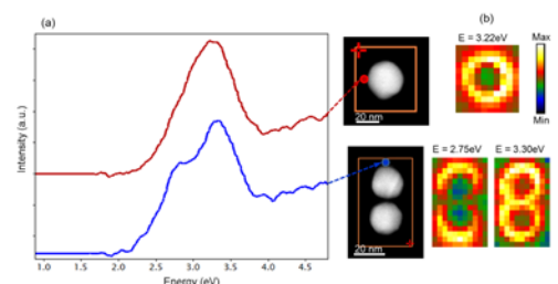
Figure 1 EEL spectra and images of EELS signal intensities in a specific energy window [5].
