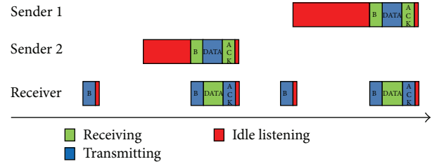
FIGURE 1: Receiver-initiated paradigm of communication. The sender is passively listening to the channel for a beacon (B) that initiates the communication. Idle listening indicates a source of energy consumption where the node is active, receiving, while the other side of the link is in sleeping mode.
