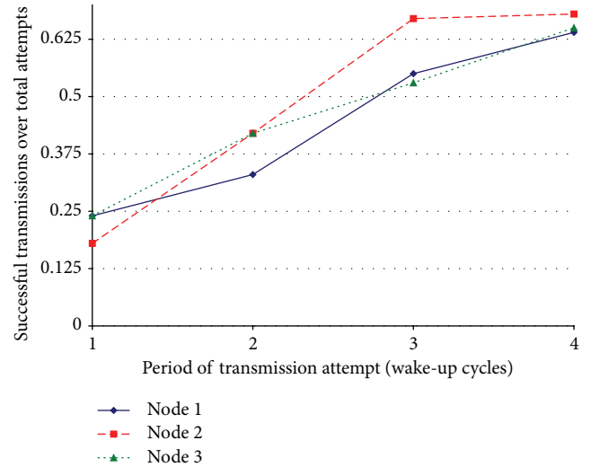
FIGURE 12: The ratio of successful transmissions over the total number of transmission attempts indicates that AB is long-term fair.
