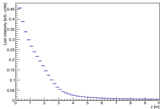
Figure 2. Histogram showing the lost neutron intensity along the straight guide as described in the text.
