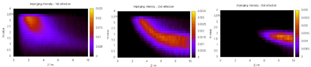
Figure 4. Histograms showing the minimum m -value required for a reflection, as a function of the position z along guide in a simulation of the 10 m straight guide described in the text. The color scale indicates the bin intensity. Note that the simulation was carried out using a m = 2 guide, which is seen to cause significant intensity loss in the beginning of the guide.
