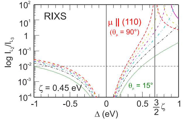
FIG. 3 (color online). Ratio of the L_2/L_3 spin-flip intensity ratio in the crossed-polarized channel as a function of the tetragonal crystal field splitting \Delta ranging from -1 to 1 eV, for a given value of the SOC constant ( \zeta = 0.45 eV). Different line styles correspond to values of \theta_\mu from 90^\circ to 0^\circ in steps of 15^\circ .
