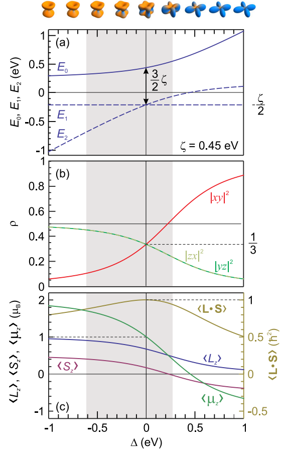
FIG. 1 (color online). \Delta dependence of (a) eigenvalues of Eq. (1) (blue lines), (b) the ground state orbital occupancies of the |xy, -\rangle (red), |yz, +\rangle (green), and |zx, +\rangle (yellow line) states, and (c) the expectation values of the orbital ( \langle L_z \rangle , blue), spin ( \langle S_z \rangle , purple) and total ( \langle \mu_z \rangle , green) magnetic moment components along z in units of \mu_B , and expectation value of the angular part of the spin orbit coupling ( \langle \mathbf{L} \cdot \mathbf{S} \rangle , yellow line) in units of \hbar^2 . The continuous blue line in panel (a) represent the ground state energy in the hole representation. The corresponding wave function [according to Eq. (2)] is represented at the top: blue and orange represent the contributions of the |xy, -\rangle and (|yz, +\rangle - i|zx, +\rangle)/\sqrt{2} states, respectively. The shaded area in all panels represents the range of \Delta values, for which the L_2/L_3 RXMS intensity ratio is smaller than 0.01 (see Fig. 2).
