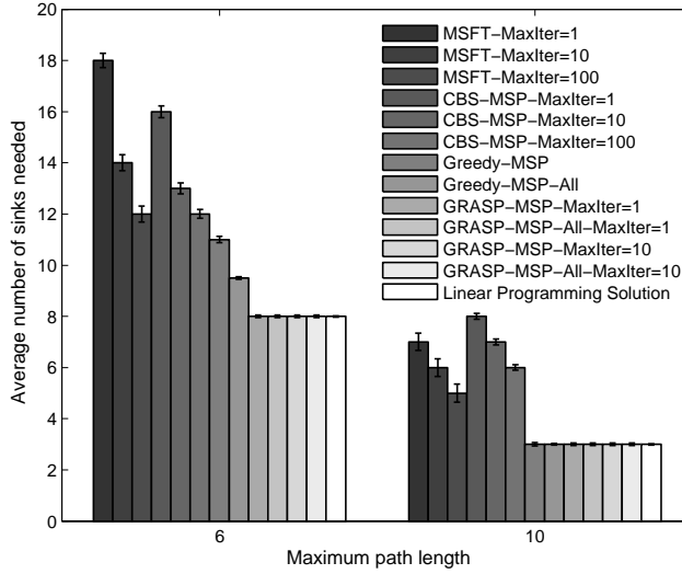
Fig. 2 Average number of sinks needed for multiple sink placement algorithms versus maximum path length
