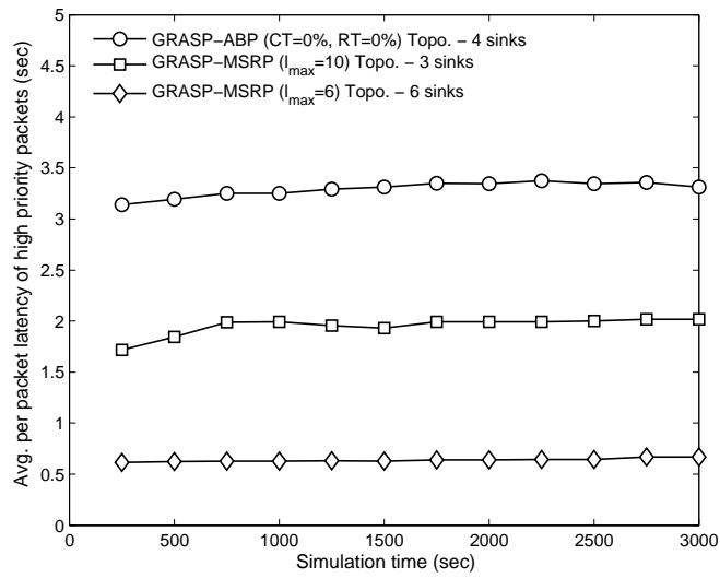
Fig. 23 Latency where a node dies every 250 seconds
