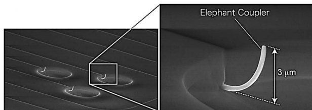
Fig. 12. SEM image of a vertically bent optical coupler, obtained by ion implantation in a silicon waveguide. The bent waveguide is 5 \mu\text{m} long, and the curvature radius is approximately equal to 3 \mu\text{m} . Reproduced from [43].
