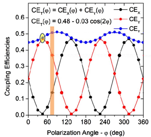
Fig. 50. Dependence of \text{CE}_x , \text{CE}_y , and \text{CE}_T on the input-beam polarization angle. Adapted from [117].
