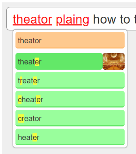
Figure 2: Sample spelling corrections suggested for the misspelled query keyword theator .
