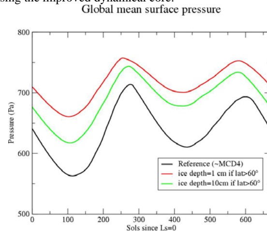
Figure 3: The major impact of high latitude subsurface ice on the CO 2 cycle simulated by the GCM. This confirms the finding of [12]
