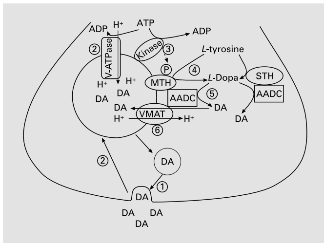
Fig. 7. A proposed model linking neuronal stimulation to activation of TH and a functional coupling between dopamine synthesis and packaging into synaptic vesicles.
