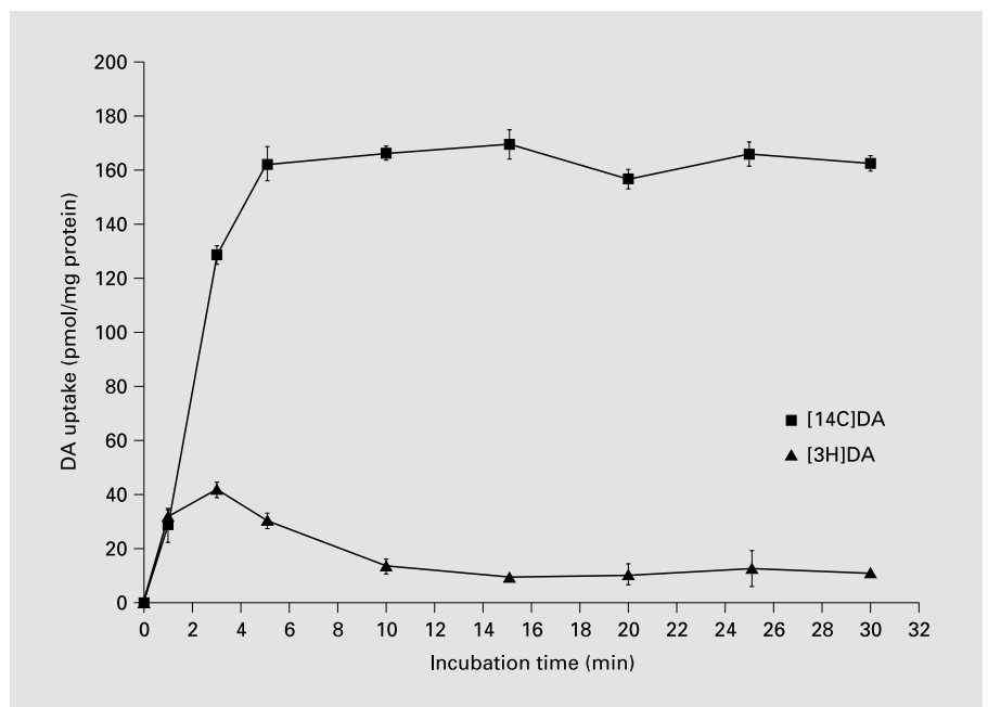
Fig. 5. A comparison of DA uptake from newly synthesized DA versus pre-existing DA. [ ^{14} C]tyrosine was used to generate newly synthesized [ ^{14} C]DA in the uptake assay system, while [ ^3 H]DA was included as pre-existing DA in uptake experiments. Uptake of DA is expressed as picomoles/milligram protein. DA uptake in the presence of CCCP was used as nonspecific uptake and was subtracted from total uptake. Values represent means and error bars represent the standard deviation of three determinations.
