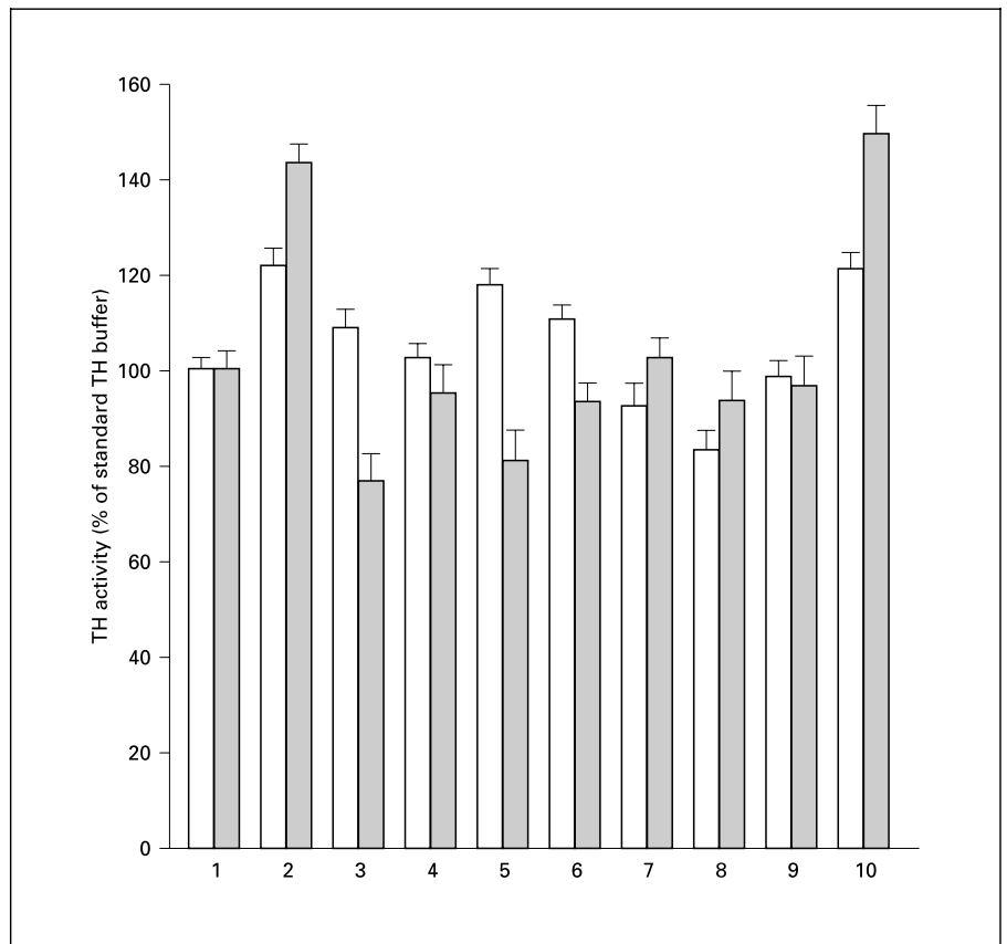
Fig. 4. Dependence of ATP activation of MTH on the proton gradient across synaptic vesicles. Effects of various proton gradient uncouplers or inhibitors on TH activity alone or on ATP activation of TH were studied as described in 'Materials and Methods'. CCCP and gramicidin were dissolved in ethanol in stock solution. The controls contained ethanol in concentrations not to exceed 1% of the incubation volume. Lane 1: control; lane 2: ATP alone (5 mM); lane 3: CCCP alone (100 \mu M); lane 4: ATP (5 mM) + CCCP (100 \mu M); lane 5: gramicidin alone (10 \mu M); lane 6: ATP (5 mM) + gramicidin (10 \mu M); lane 7: bafilomycin alone (6 \mu M); lane 8: ATP (5 mM) + bafilomycin (6 \mu M); lane 9: vanadate alone (200 \mu M); lane 10: ATP (5 mM) + vanadate (200 \mu M). Values represent means and error bars represent the standard deviation of three determinations.
