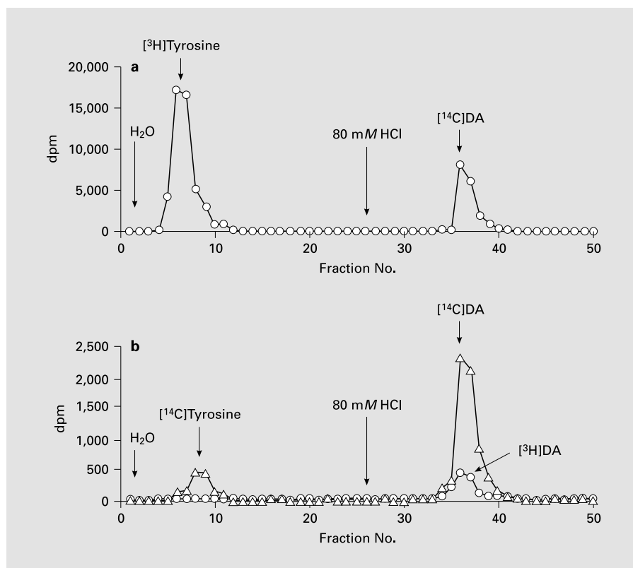
Fig. 6. Separation of tyrosine and DA on an anion exchange column. a Elution pattern of standard tyrosine (45,000 dpm) and dopamine (15,000 dpm) on an anion exchange column. Tyrosine was eluted out when washed with H 2 O (first peak), while DA was eluted later with 80 mM HCl as indicated in the second peak. b Elution pattern of the content extracted from synaptic vesicles as described in 'Materials and Methods'. The first peak corresponding to tyrosine is the nonspecifically absorbed tyrosine, the second large peak corresponding to the standard DA is newly synthesized [ 14 C]DA taken up by DA synaptic vesicles. The small peak at the same position as [ 14 C]DA is [ 3 H]DA taken up from the pre-existing [ 3 H]DA pool.
