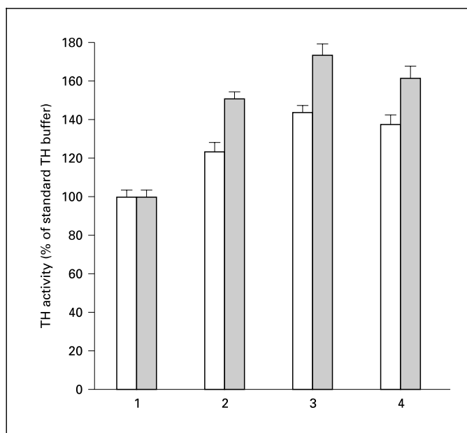
Fig. 2. Effects of protein kinase activators on TH activity. The STH and MTH samples were incubated under the following conditions. Lane 1: standard TH buffer only; lane 2: TH buffer + ATP (5 mM); lane 3: TH buffer + ATP (5 mM) + cAMP (1 mM); lane 4: TH buffer + ATP (5 mM) + CaCl 2 (1 mM). Values represent means and error bars represent the standard deviation of three determinations.
