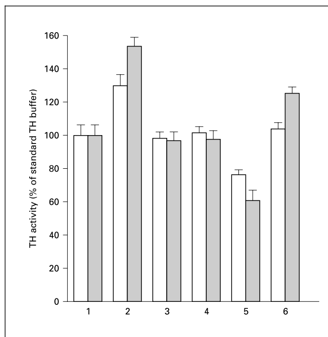
Fig. 1. Effect of ATP and protein phosphatase inhibitors on TH activity. The STH and MTH samples were prepared as described under 'Materials and Methods'. The TH samples were incubated at 37 °C for 30 min under the following conditions. Lane 1: standard TH buffer; lane 2: standard TH buffer + 5 mM ATP; lane 3: standard TH buffer + 5 mM ADP; lane 4: standard TH buffer + 5 mM AMP; lane 5: standard TH buffer + 2 mM EGTA; lane 6: standard TH buffer + phosphatase inhibitors (0.2 mM vanadate, 2 mM sodium fluoride and 0.2 mM sodium pyrophosphate). Values represent means and error bars represent the standard deviation of three determinations.
