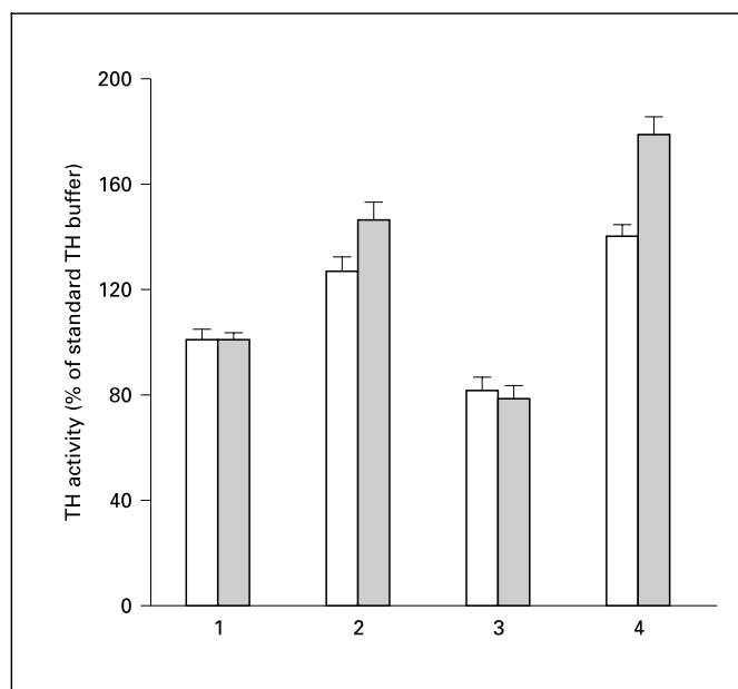
Fig. 3. Effects of phosphatase on TH activity. Both STH and MTH samples were treated with CIP as described in 'Materials and Methods'. Lane 1: TH buffer as control; lane 2: TH buffer + 5 mM ATP; lane 3: treatment with CIP; lane 4: same as lane 3, followed by addition of 5 mM ATP. Data are expressed as the mean \pm the standard deviation. Values represent means and error bars represent the standard deviation of three determinations.
