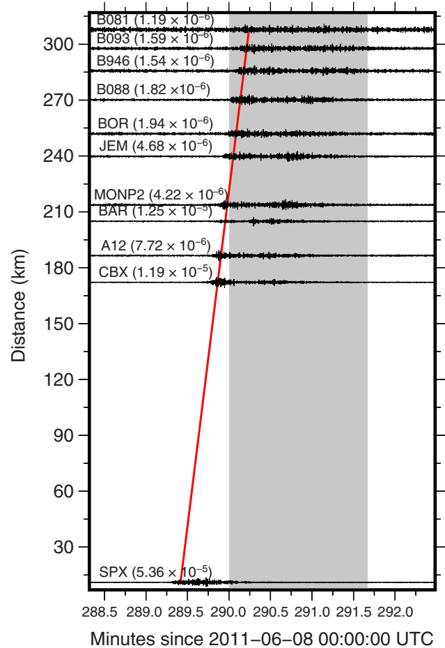
Figure 10. Vertical ground motions as a function of time (UTC) caused by a regional unregistered event that occurred in southern Baja California on 8 June 2011. Stations are sorted according to their distance from an arbitrary point just south of station BC.SPX in Baja California, the southernmost station that recorded this event. Diagonal line indicates propagation velocity of 6 km/s. Stations names and peak ground velocity ( \text{cm}/\text{s} ) are indicated above each trace. Other symbols are as in Figure 9. The color version of this figure is available only in the electronic edition.
