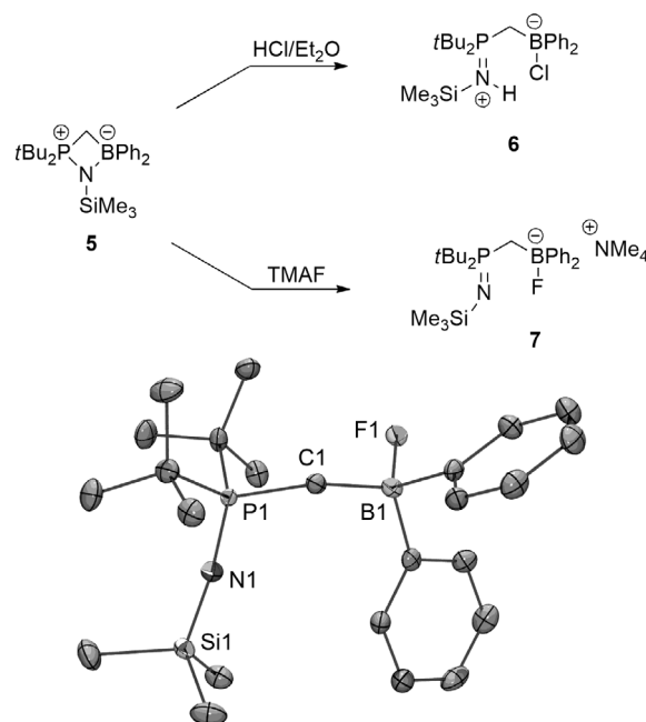
Scheme 4. The reaction of 5 with HCl and TMAF (top) and the molecular structure of 7 (bottom; ellipsoids at 50% probability, hydrogens Me 4 N cation and a second ion pair of 7 are omitted for clarity). Selected bond lengths [Å] and angles [°] for 7 (structural parameter for the second crystallographic independent molecule in brackets): P1–N1 (1.543(3) [1.545(3)]), B1–F1 1.470(4) [1.473(4)], N1–Si1 1.653(3) [1.648(3)]; P1–C1–B1 131.9(2) [130.9(2)], P1–N1–Si1 171.5(2) [174.6(2)], \Sigma(\text{C–B1–C}) 331 [332].
