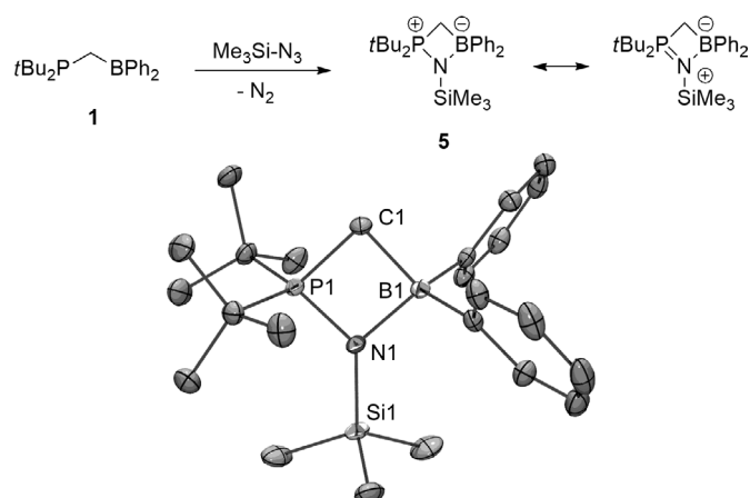
Scheme 3. The reaction of 1 with TMS–N 3 (top) and the molecular structure of 5 (bottom; ellipsoids at 50% probability, hydrogens are omitted for clarity). Selected bond lengths [Å] and angles [°] for 5 : P1–N1 1.6366(11), B1–N1 1.6802(18), N1–Si1 1.7348(12); P1–N1–B1 90.96(7), B1–N1–Si1 132.33(8), Si1–N1–P1 135.66(7).
