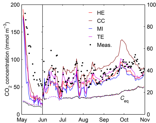
Figure 4. Simulated CO 2 concentrations (mmol m -3 ) in the surface layer (0–0.5 m) obtained with each GEM and the daily averages of the automatic measurements at 0.2 m in Lake Kuivajärvi in May–October 2013. Also shown are the atmospheric equilibrium concentrations of CO 2 ( C_{eq} ) obtained from the simulations (dotted colored lines) and calculated from the measured atmospheric CO 2 concentration and surface water temperature (solid black line). Note the different vertical scales in May and in June–October.
